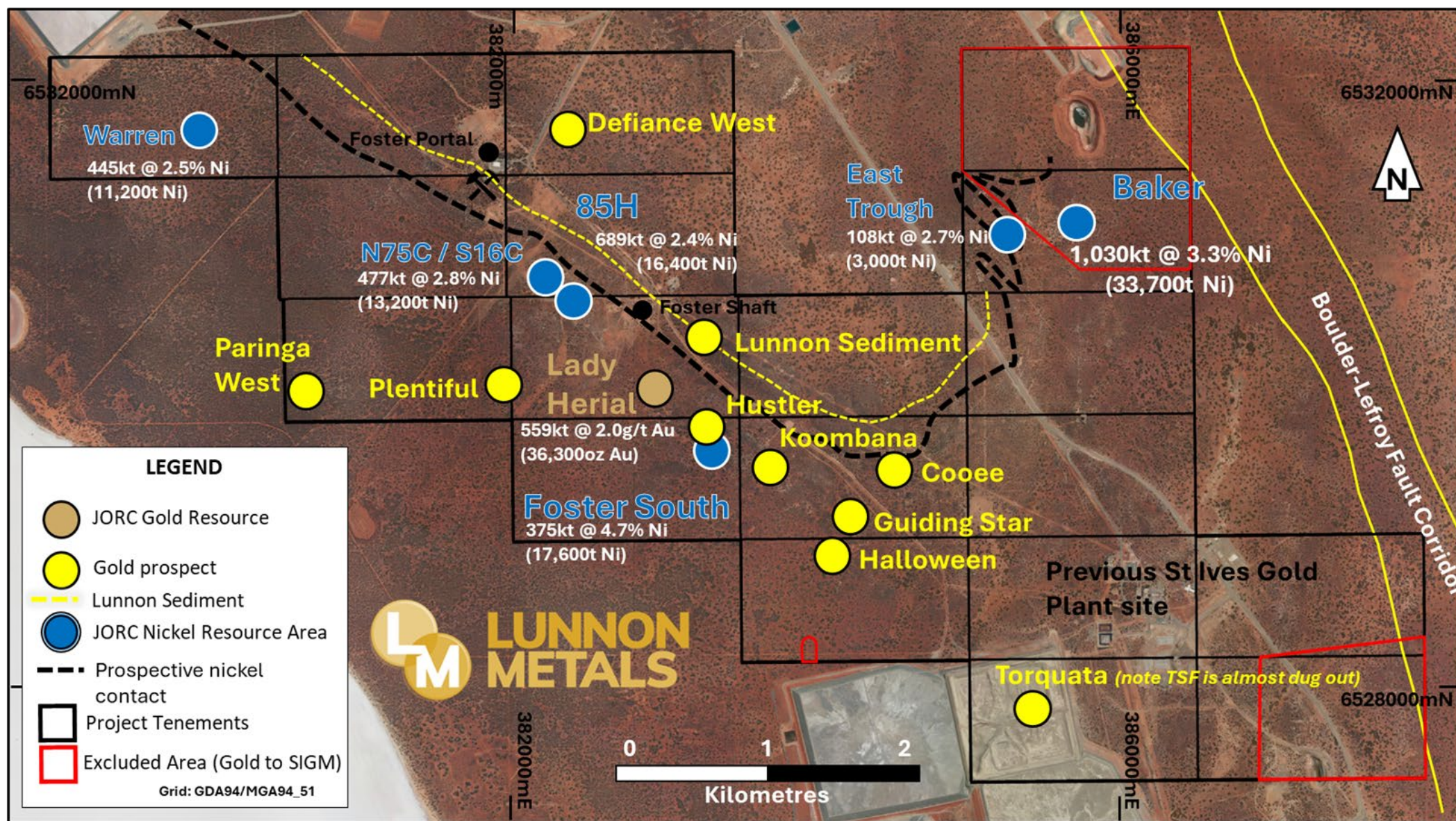
Figure 8: Foster-Baker Project Area showing select high-ranking gold prospects, gold & nickel Mineral Resource 9 positions.
