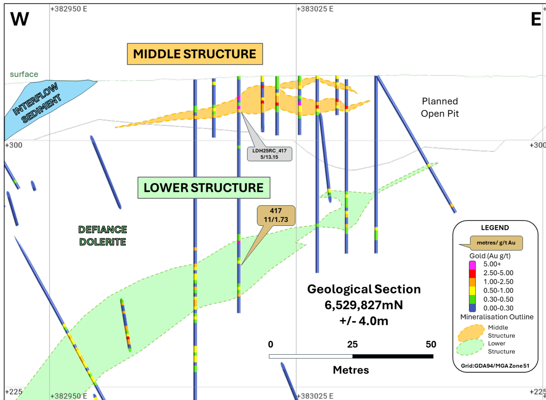
Figure 6: Section 6,529,827mN (looking north +/- 4m) illustrating the results reported today (gold call-outs).
