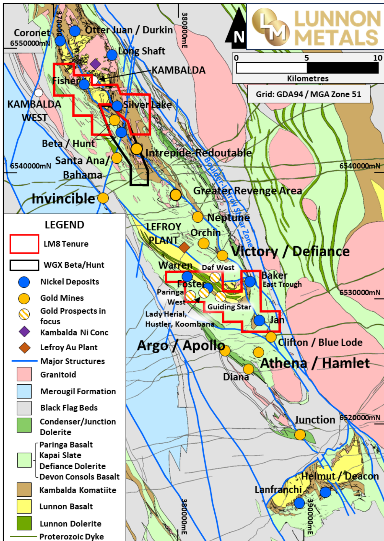
Figure 9: Location of the KGNP (red outlines) at the local Kambalda/St Ives scale; showing surface geology and structure of this significant Australian gold camp.
