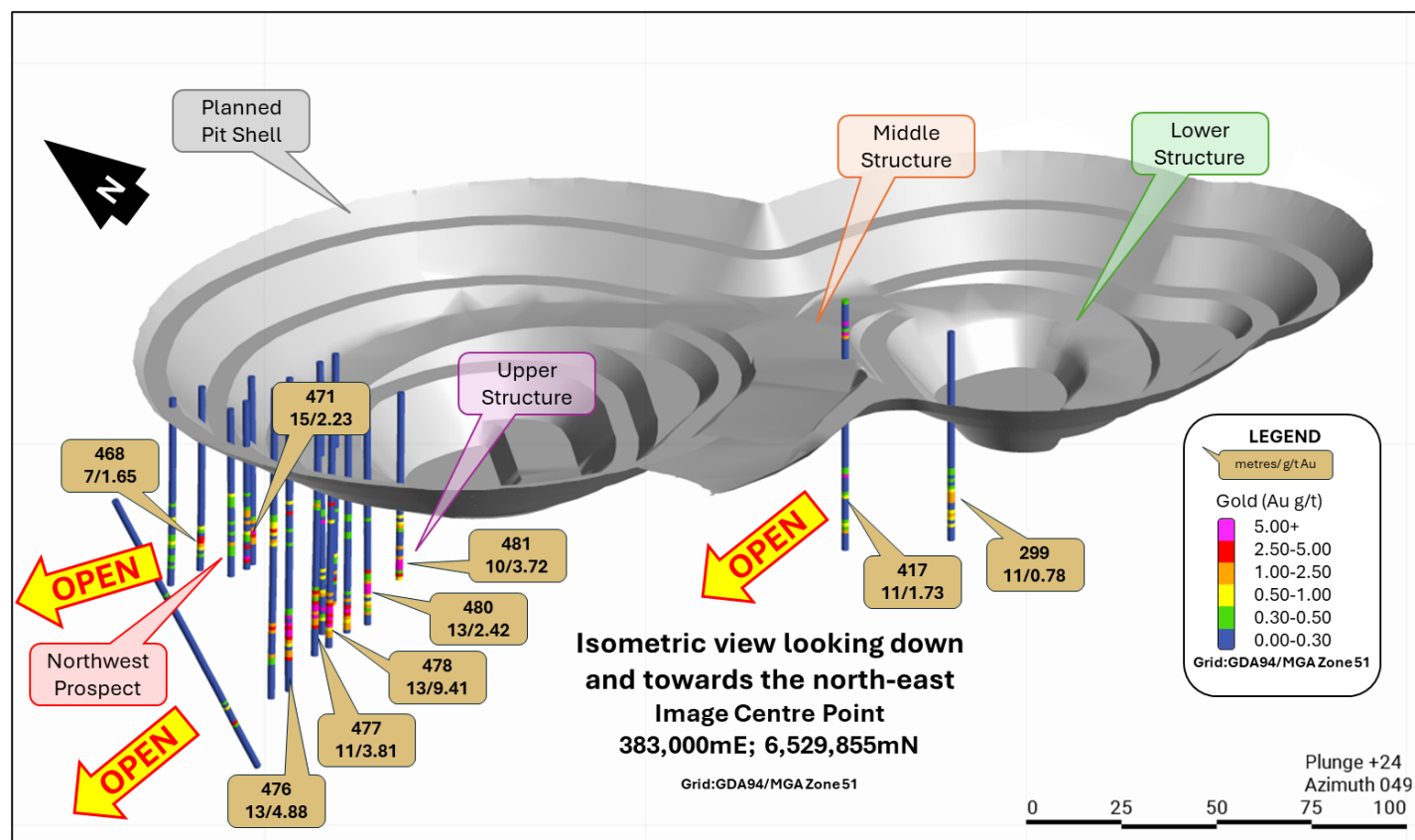
Figure 1: Isometric view of the Lady Herial open pit development area illustrating the results reported today and the opportunity that remains open down plunge on the NWP and the Upper Structure.
