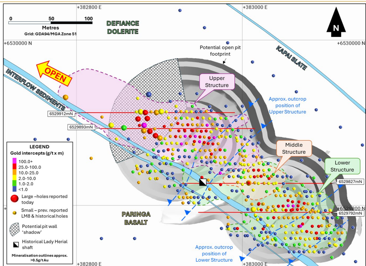
Figure 2: Plan view of the Lady Herial open pit development area illustrating the Upper Structure results reported today (larger spheres) and prior reported results (smaller spheres) together with a representation of the 'shadow' along the northwest wall of the planned pit (hatched area).
