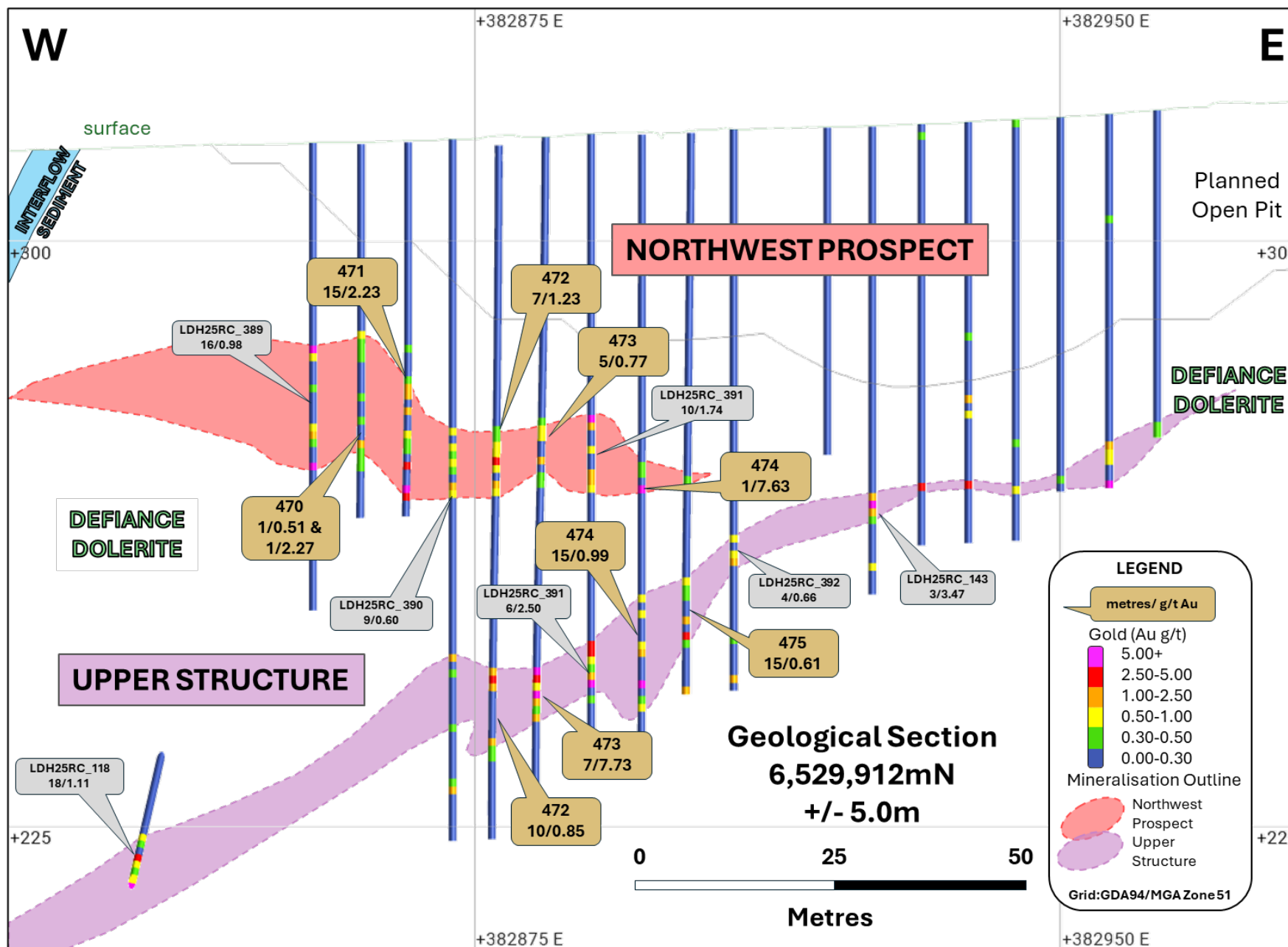
Figure 4: Section 6,529,912mN (looking north +/- 5m) illustrating the results reported today (gold call-outs) and select prior reported results (grey call-outs).
