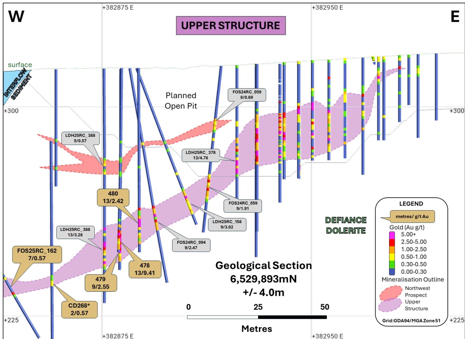
Figure 5: Section 6,529,893mN (looking north +/- 4m) illustrating the results reported today (gold call-outs) and select prior reported results (grey call-outs).
