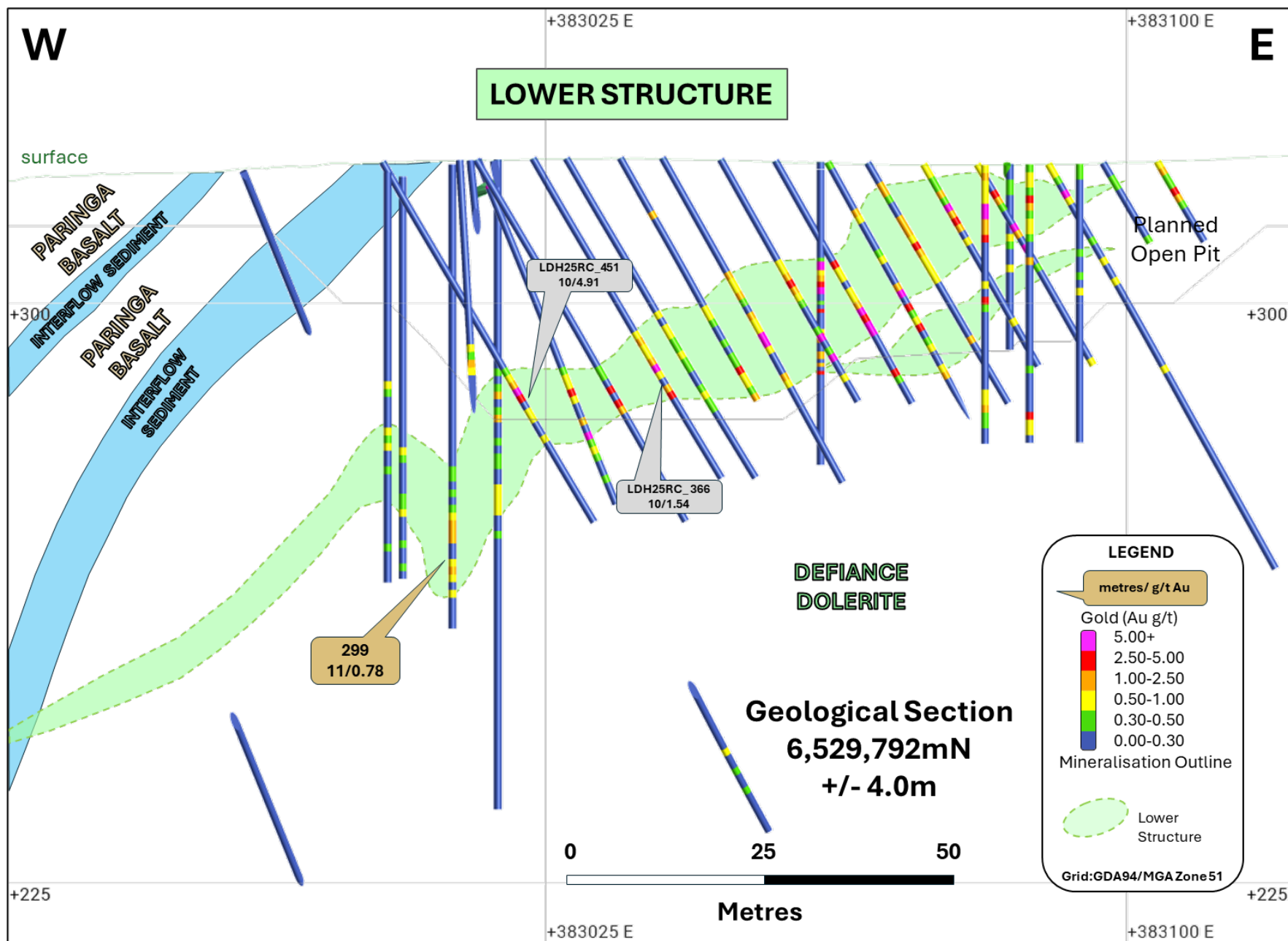
Figure 7: Section 6,529,792mN (looking north +/- 4m) illustrating the results reported today (gold call-outs).
