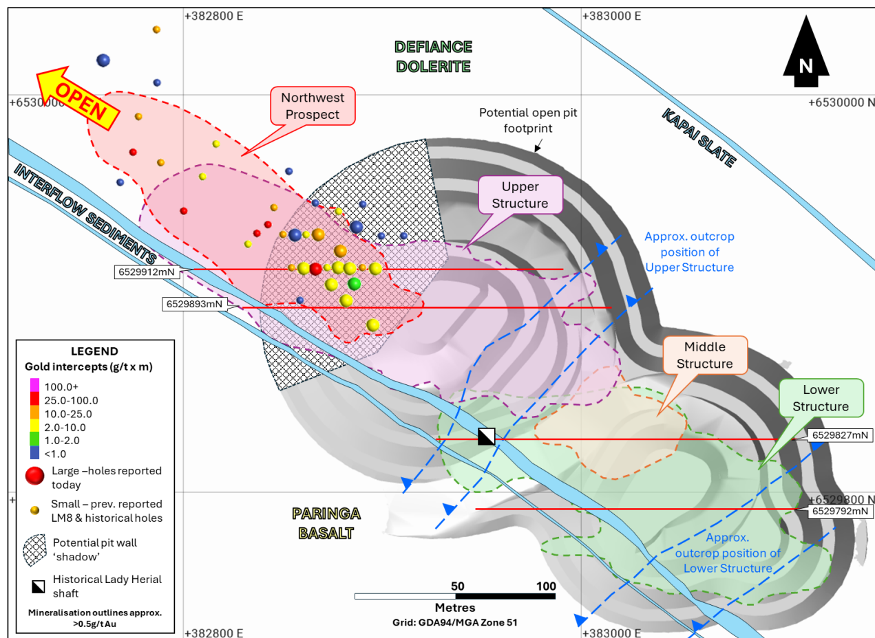
Figure 3: Plan view of the Lady Herial open pit development area illustrating the NWP results reported today (larger spheres) and prior reported results (smaller spheres) together with a representation of the 'shadow' along the northwest wall of the planned pit (hatched area).
