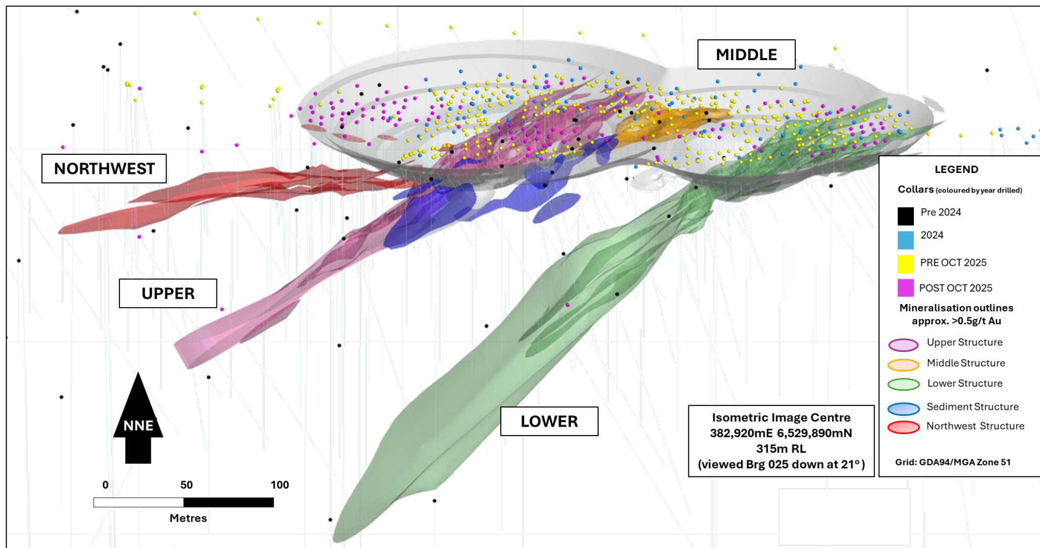
Figure 7: Isometric view, looking down and toward the NNE, of the Lady Herial gold deposit illustrating all drilling coded by period drilled and the open pit design.
