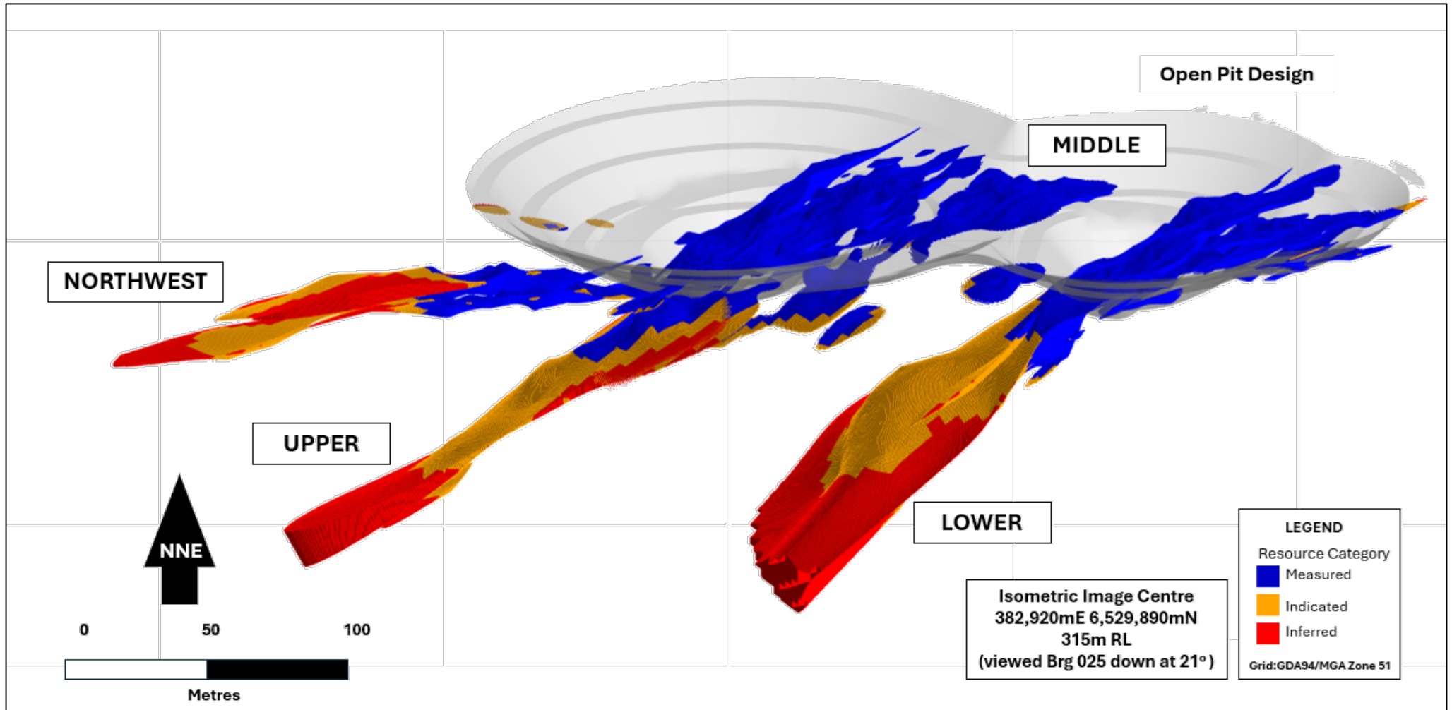
Figure 9: Isometric view, looking down and toward the NNE, of the Lady Herial gold deposit illustrating the Upper, Lower, Middle and Northwest Structures coloured by Mineral Resource classification categories.
