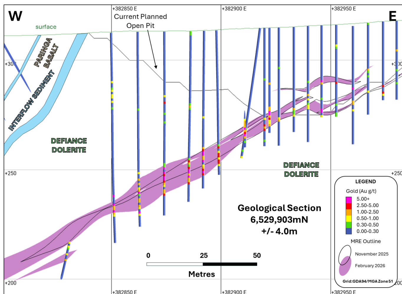
Figure 6: Geological cross section through the Upper Structure summarising changes in the modelled high grade lenses against the November 2025 MRE outline (with current open pit shell).
