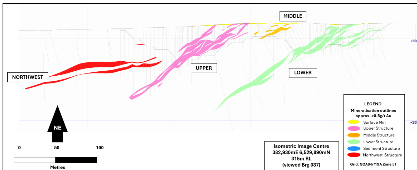
Figure 5: Geological long section looking towards the north-east showing Upper Structure, Middle, Lower and Northwest Structures and a slice through the open pit shell.
