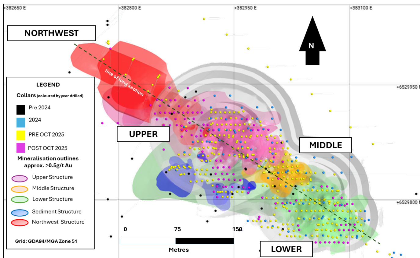
Figure 4: Plan view at the Lady Herrial deposit scale, illustrating all drilling (by period drilled) along with location of long section shown in Figure 5.
