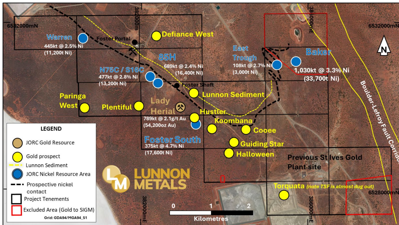
Figure 3: Foster-Baker Project Area showing select high-ranking gold prospects, gold & nickel Mineral Resource 7 positions.
