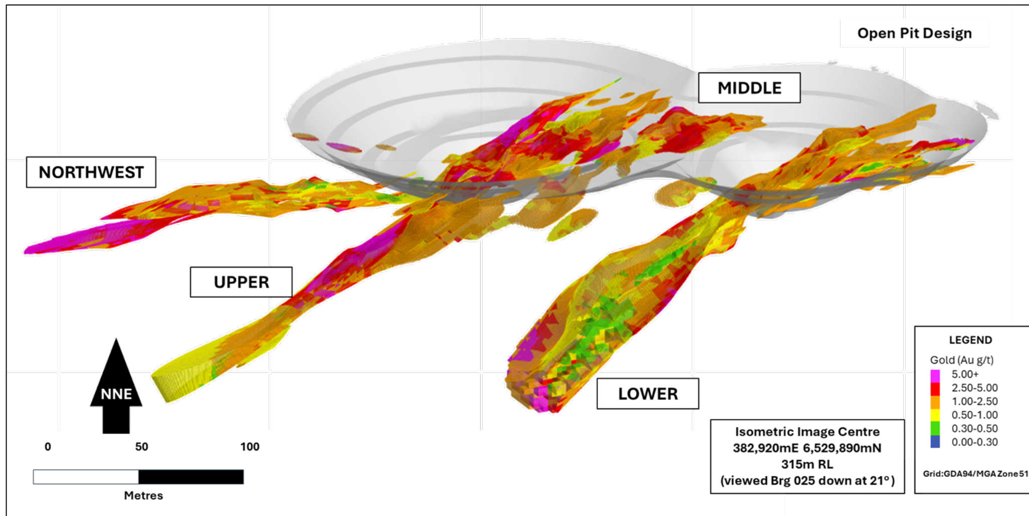
Figure 8: Isometric view, looking down and toward the NNE, of the Lady Herial gold deposit illustrating the Upper, Lower, Middle and Northwest Structures coloured by estimated gold grade (g/t Au).
