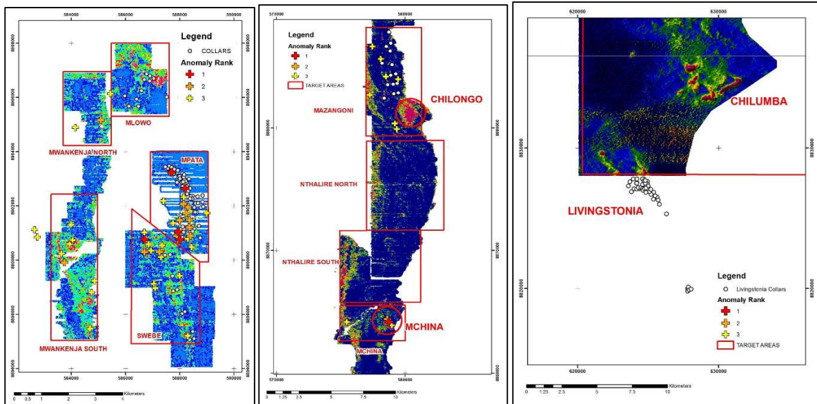
Figure 7: Kayelekera Project Exploration Target Areas
