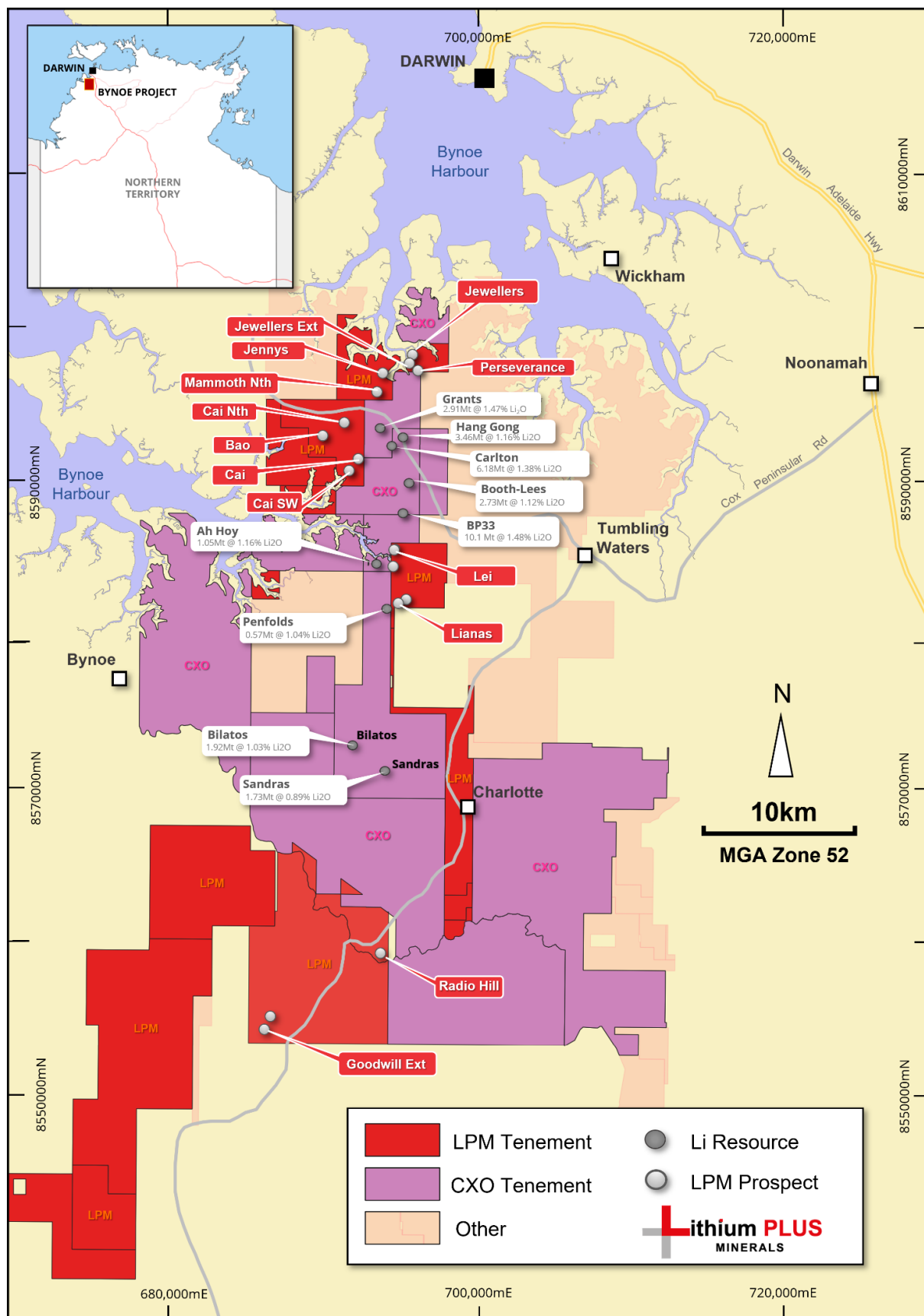
Figure 4: Bynoe Project Location map and pegmatite prospects.
