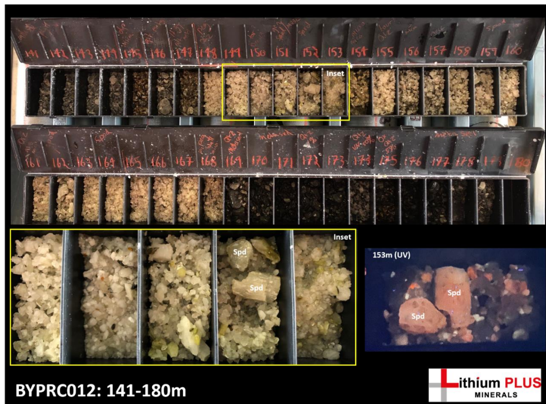
Figure 1: High grade intersection in RC drill chips from BYPRC012 (140 to 180m)
