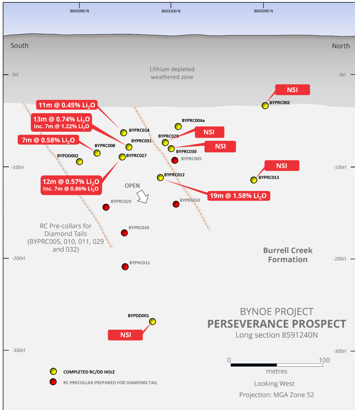
Figure 2: North-South long section with drill hole pierce points and grade intersections in RC drill chips.
