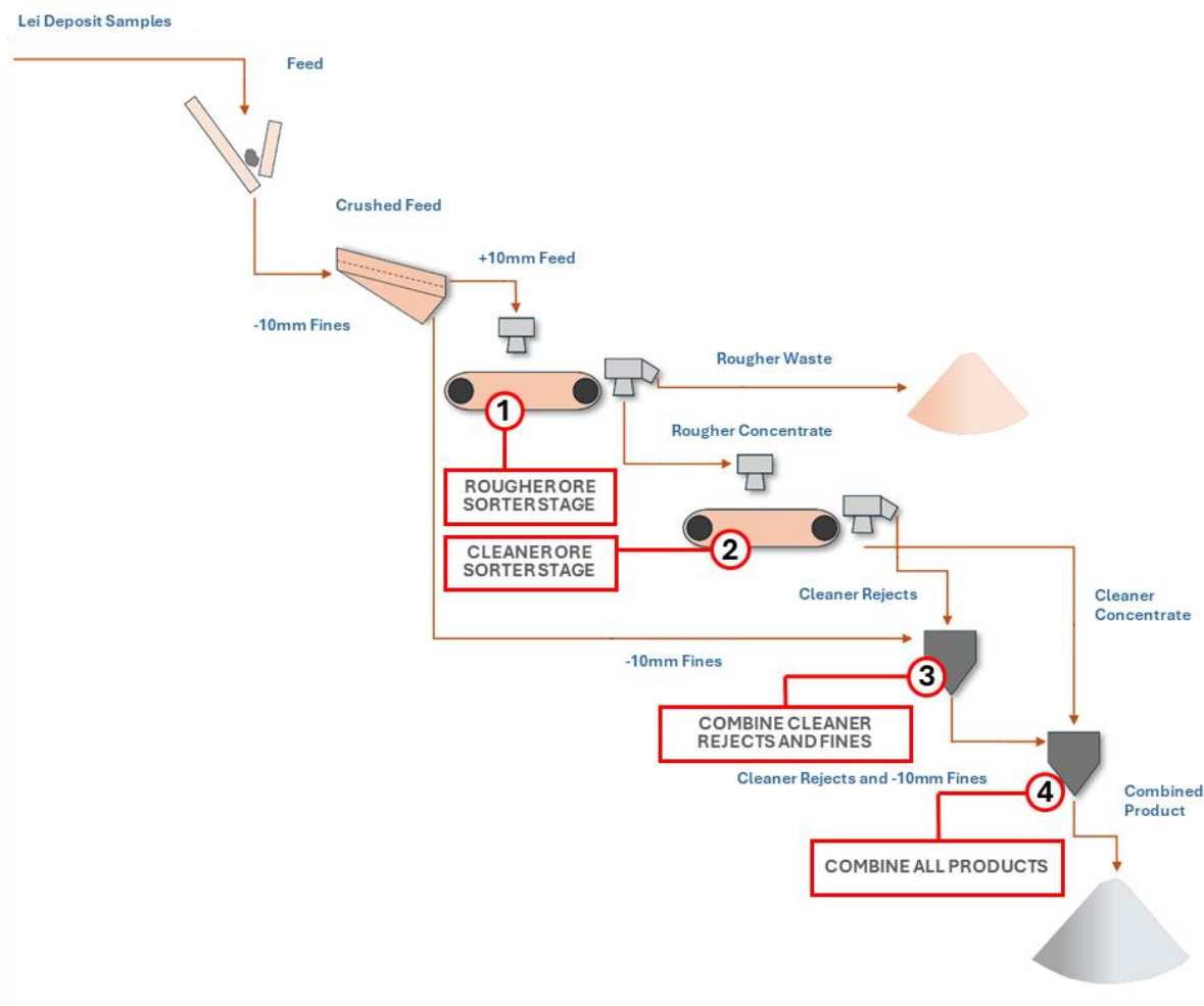
Figure 3: Sorter test work schematic
