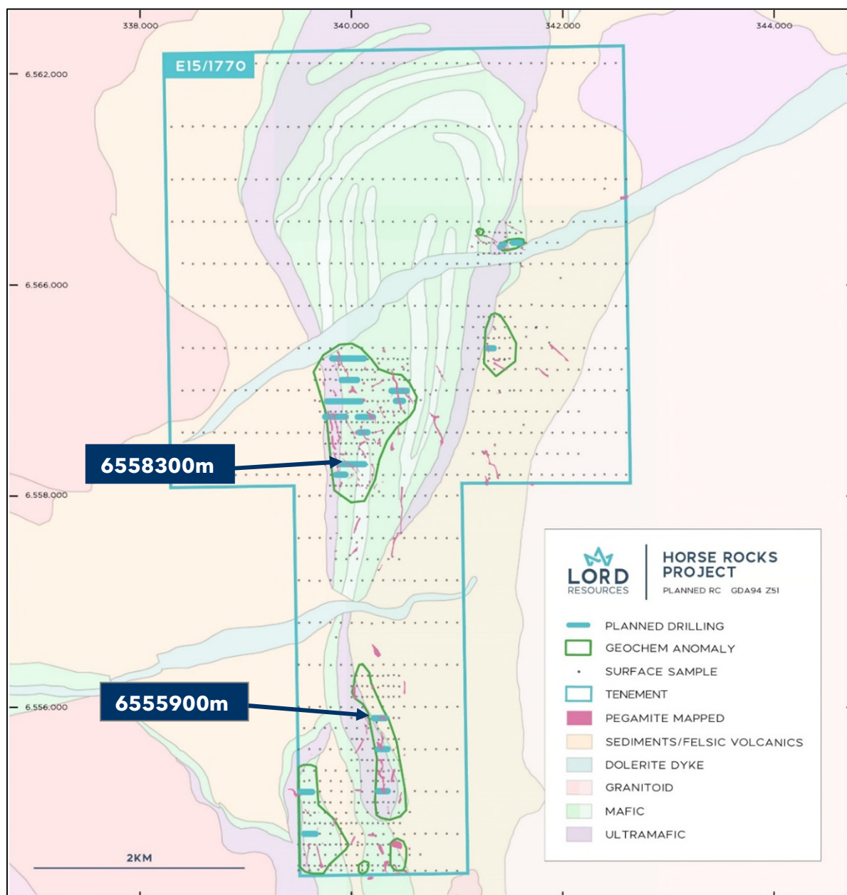
Figure 6 RC drilling overlain geochemical samples and interpreted geology
