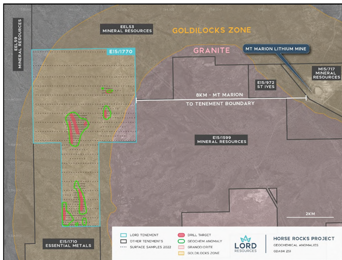
Figure 1 Horse Rocks Project showing proximity to MRL and ESS
