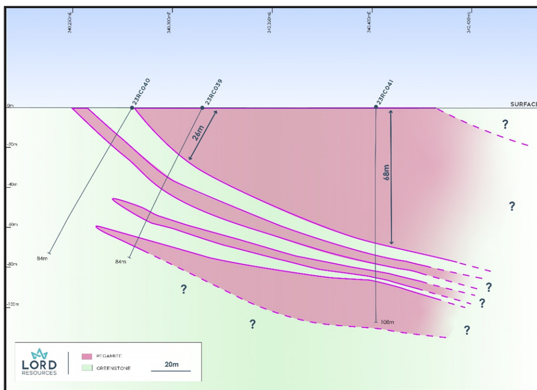
Figure 2 Simplified cross section from 6555900mN showing wide zones of pegmatite.
