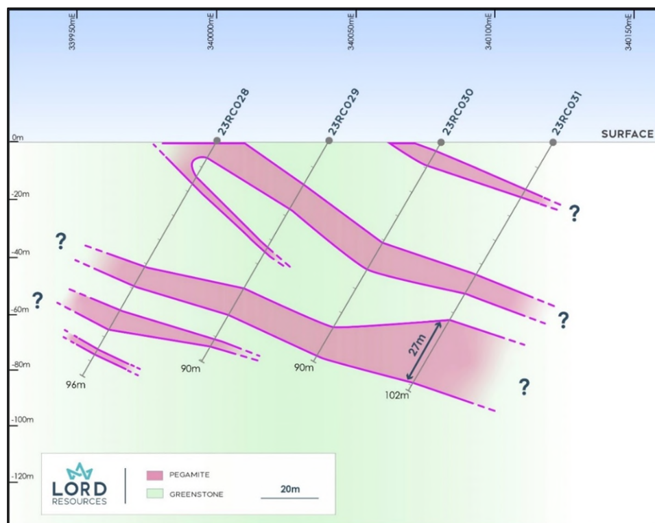
Figure 3 Simplified cross section from 6558300mN showing wide zones of pegmatite.
