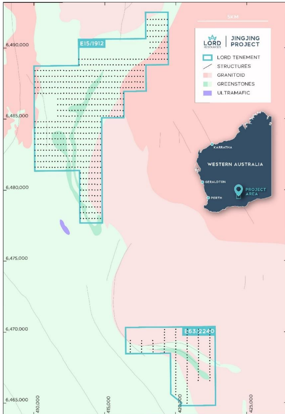
Figure 2 Simplified geology of the Jingjing project, with soil sample locations.
