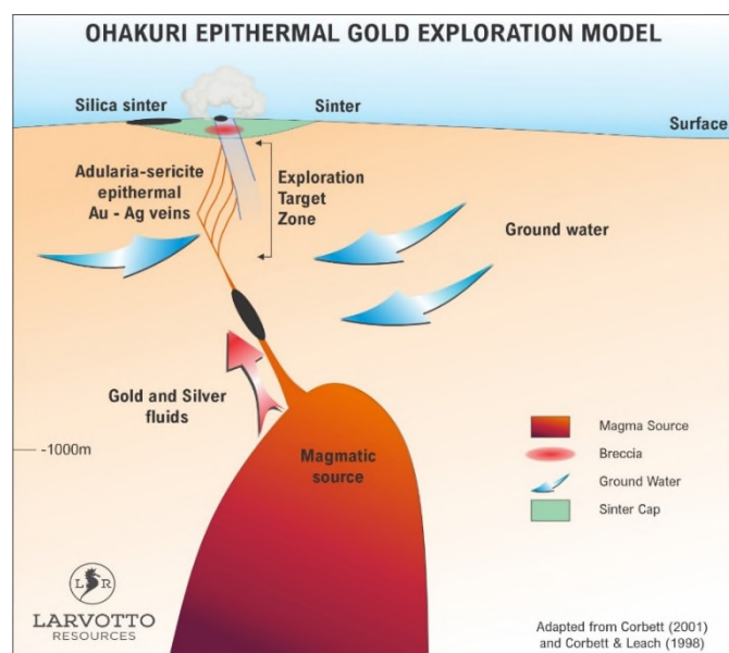
Figure 2. Ohakuri epithermal gold exploration model
