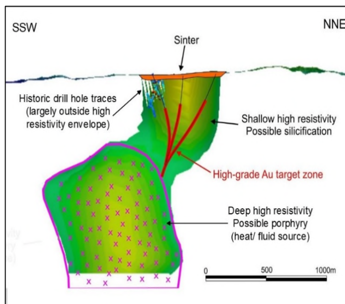
Figure 3. Vertical slice through ESCAN geophysics with geological interpretation
