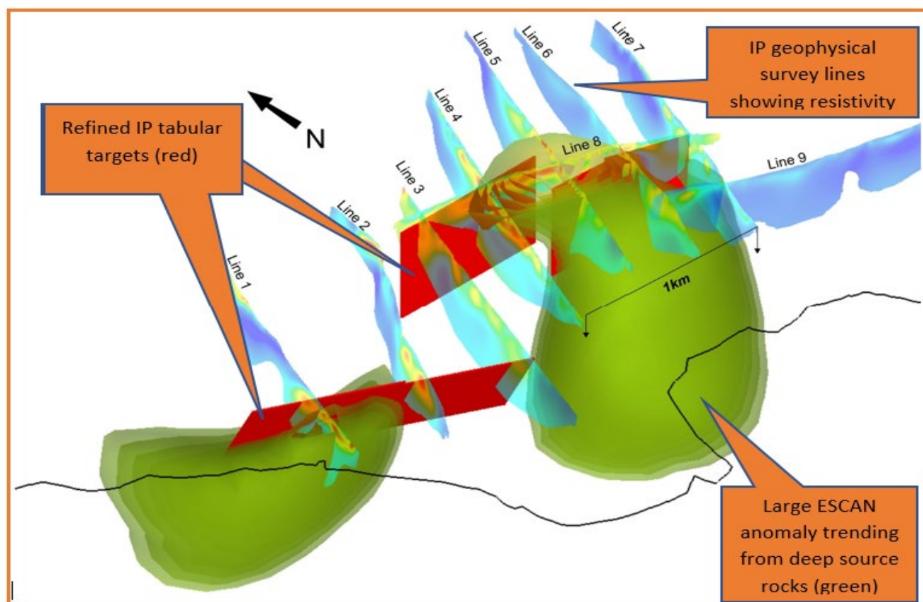
Figure 5 3D image showing ESCAN and IP survey lines with potential gold feeder target zones
