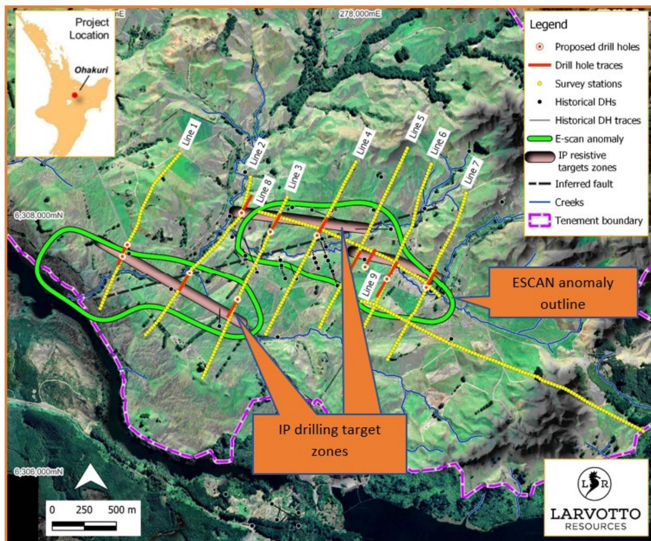
Figure 1 Location diagram showing new survey lines and outline of historic broad ESCAN, historic drilling and proposed new drill holes
