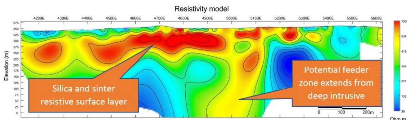
Figure 2 Survey line 6 (across strike) showing potential feeder zone extending to surface from a deep intrusive source
