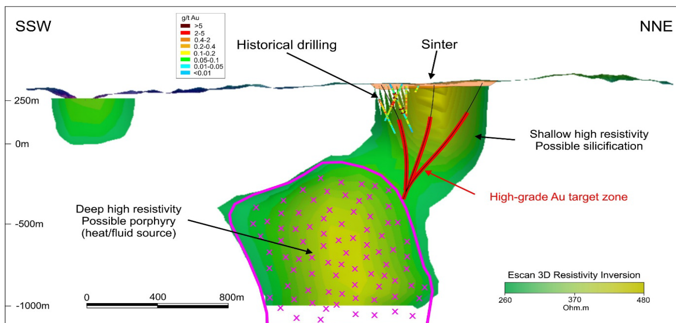
Figure 4 Historic ESCAN anomaly showing deep source and offset from previous drilling
