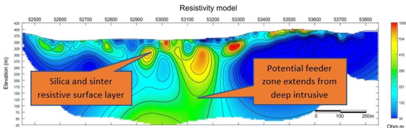
Figure 3 Survey line 8 (along strike) showing resistive potential feeder zone extending to depth
