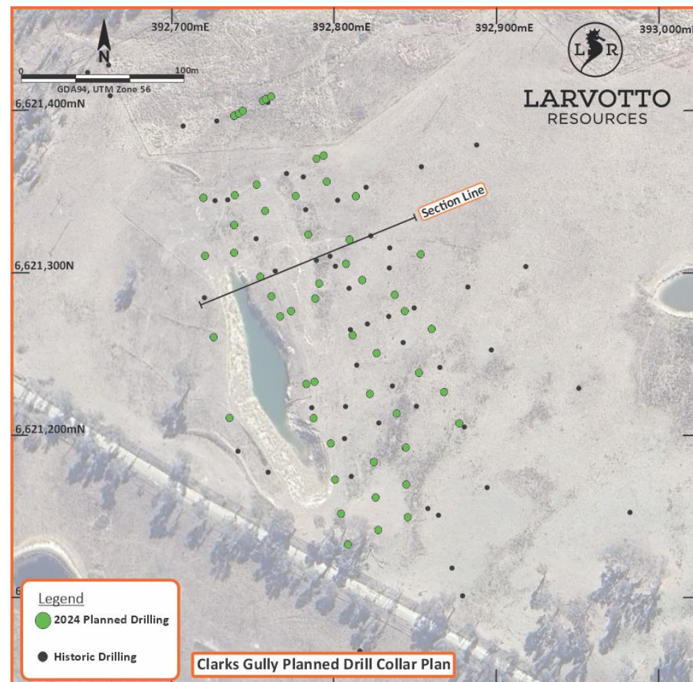
Plan view of drilling for Clarks Gully
