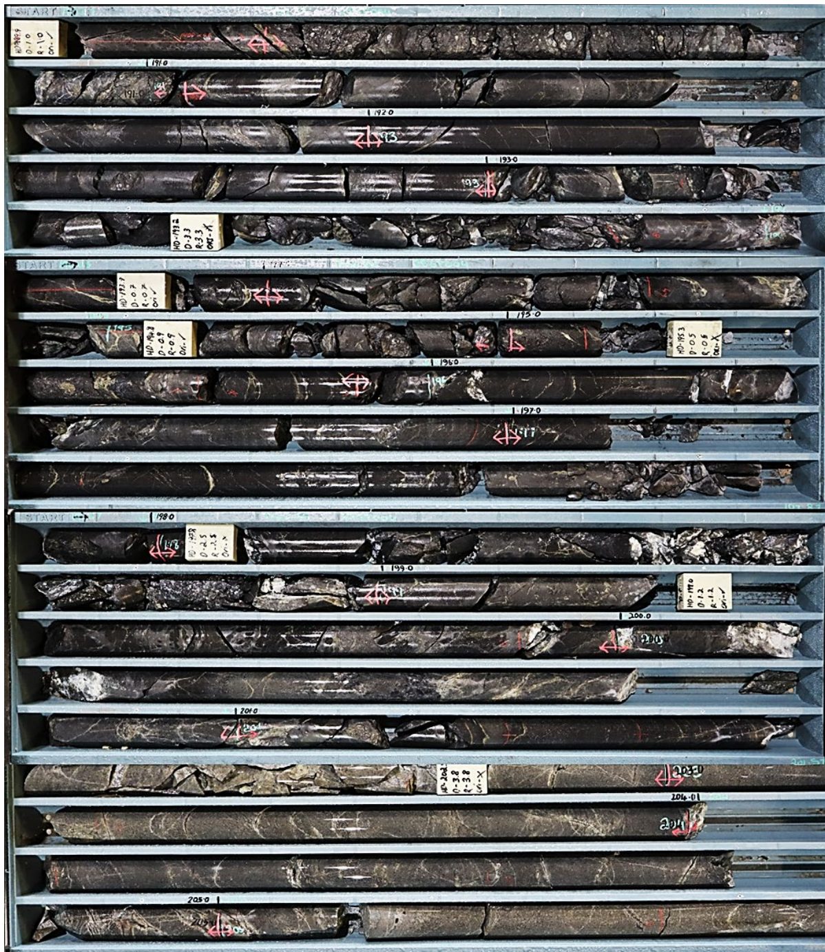
Figure 3. Drill core photos (wet) of the elevated Mo-Te-Sb±TGC geochemical zone (~189-202m) in hole 25GT004. Plutonic has logged sulphide veining in graphite-rich (hydrothermal) sedimentary rock coincident with this zone. Downhole length, true width not known.
