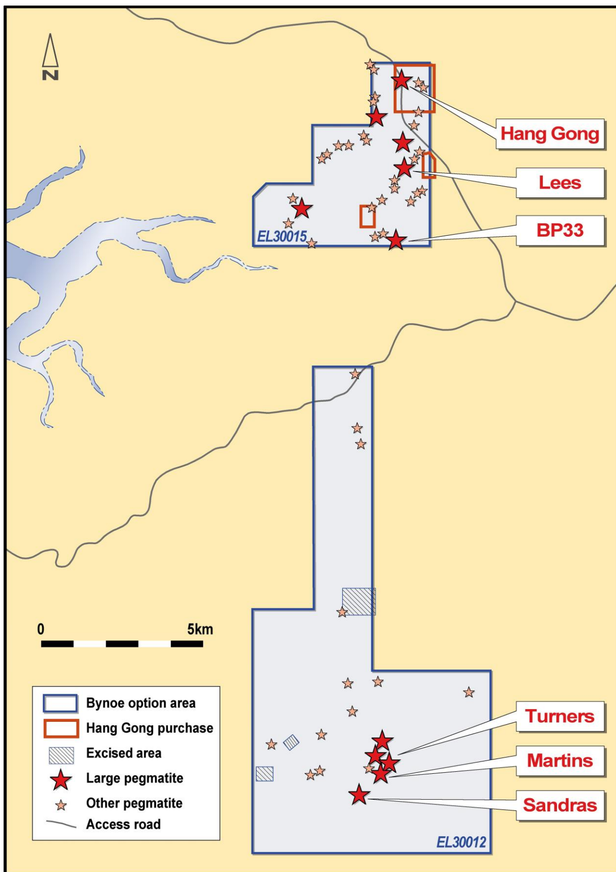
Figure 2: Bynoe Project – Tenure and pegmatite occurrences
