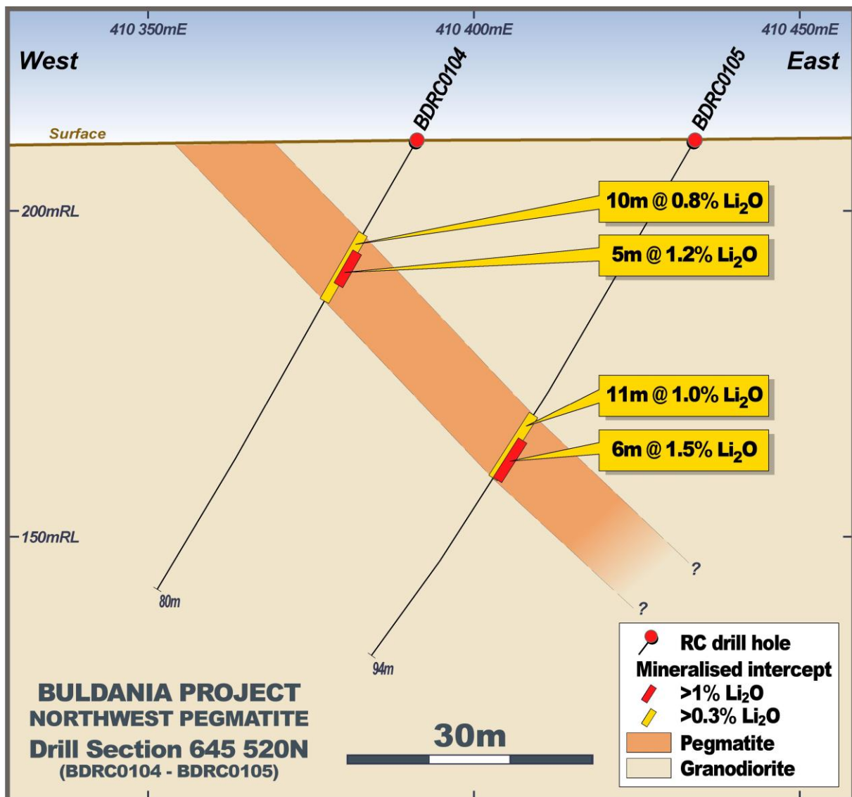
Figure 4: NW Pegmatite Area – Drill section showing recent lithium results (see Figure 4 for location).
