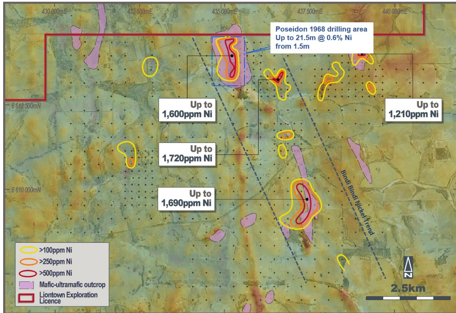
Figure 4: Moora Project/Bindi Bindi Nickel Trend: Regional aeromagnetic image showing Liontown auger sampling over aerial photograph
