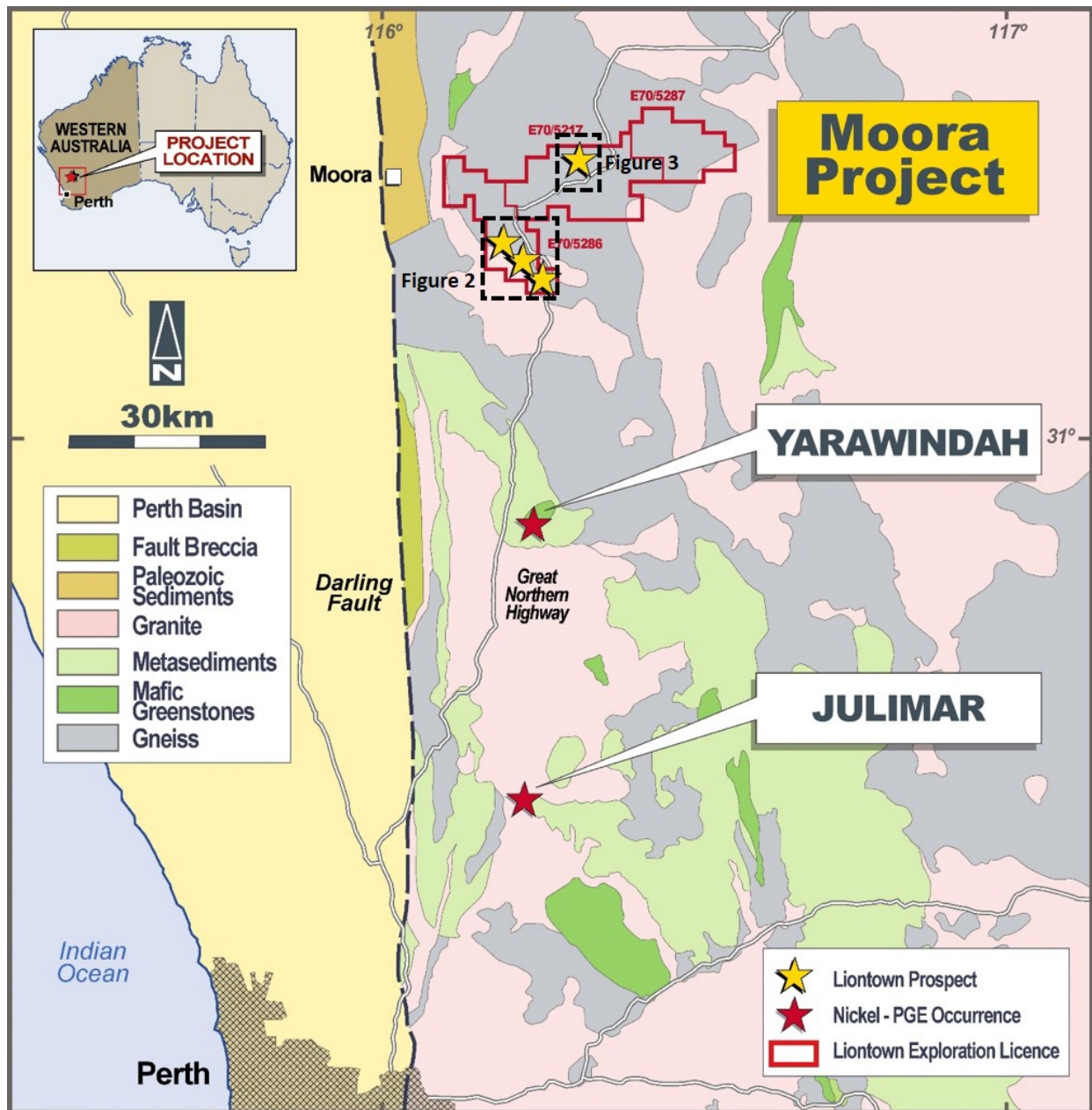
Figure 2: Moora Project: Location plan and regional geology.
