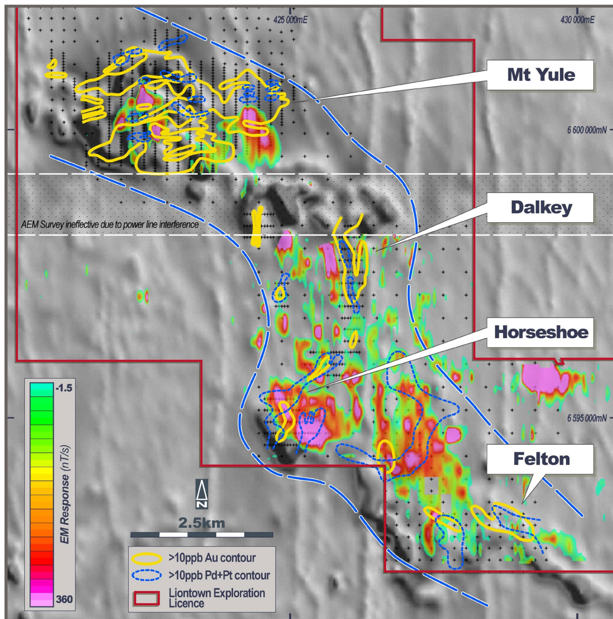
Figure 3: Moora Project/Mt Yule-Felton Corridor: Gold-PGE and airborne EM anomalies over grey-scale magnetic image with darker grey indicating potential mafic/ultramafic intrusions
