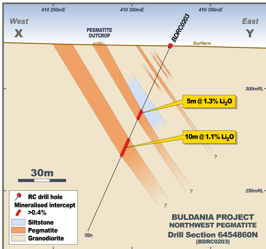
Figure 8: Buldania Project: BDRC0203 Northwest Prospect geological cross-section with lithium mineralised pegmatites.
