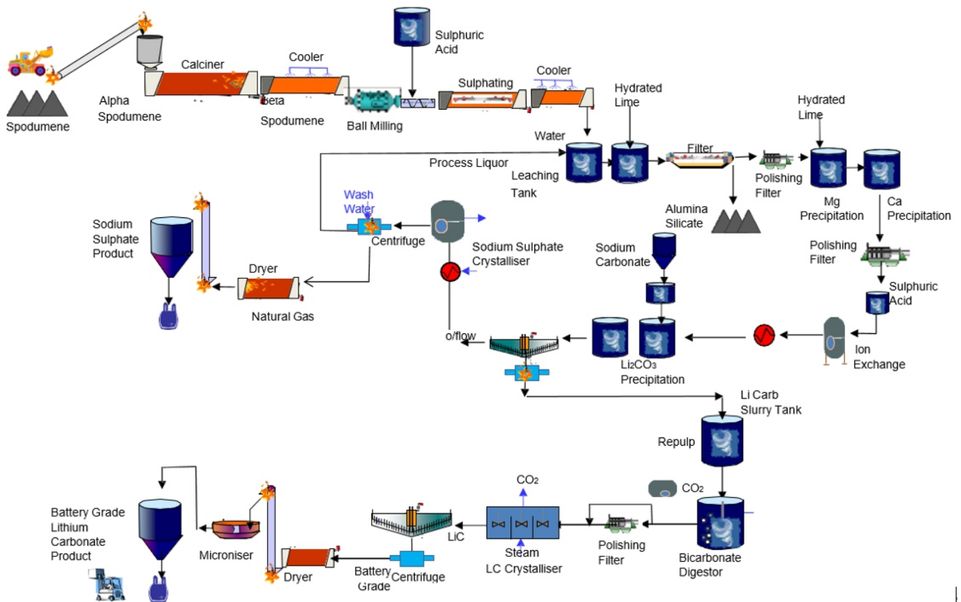
Figure 3: Process Flow Diagram, QLPH Lithium Refinery
