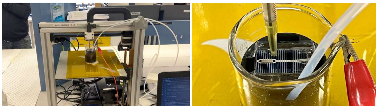
Figure 2 – Jet Electrochemical Silver Extraction Probe
