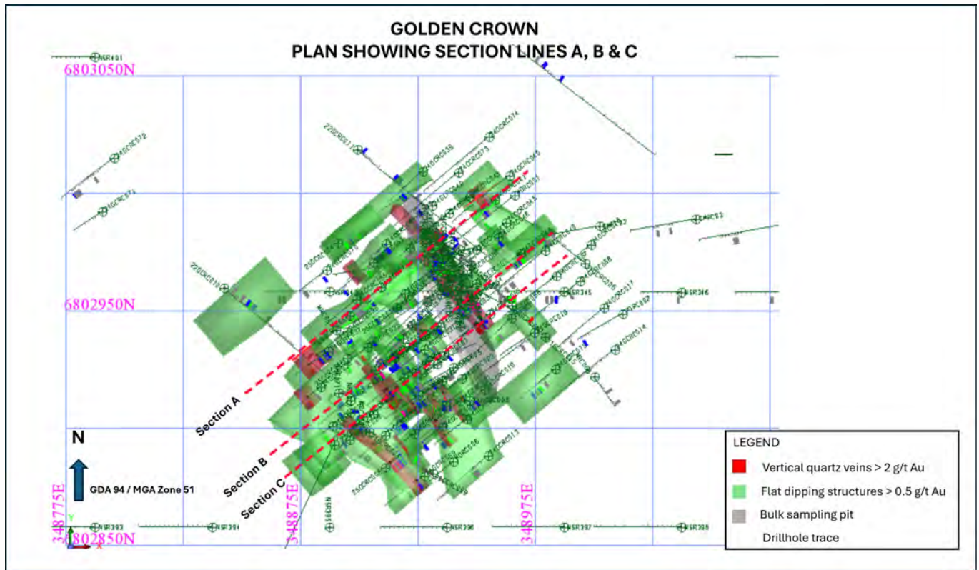
Figure 9: Golden Crown Mineralisation and CS Lines.
