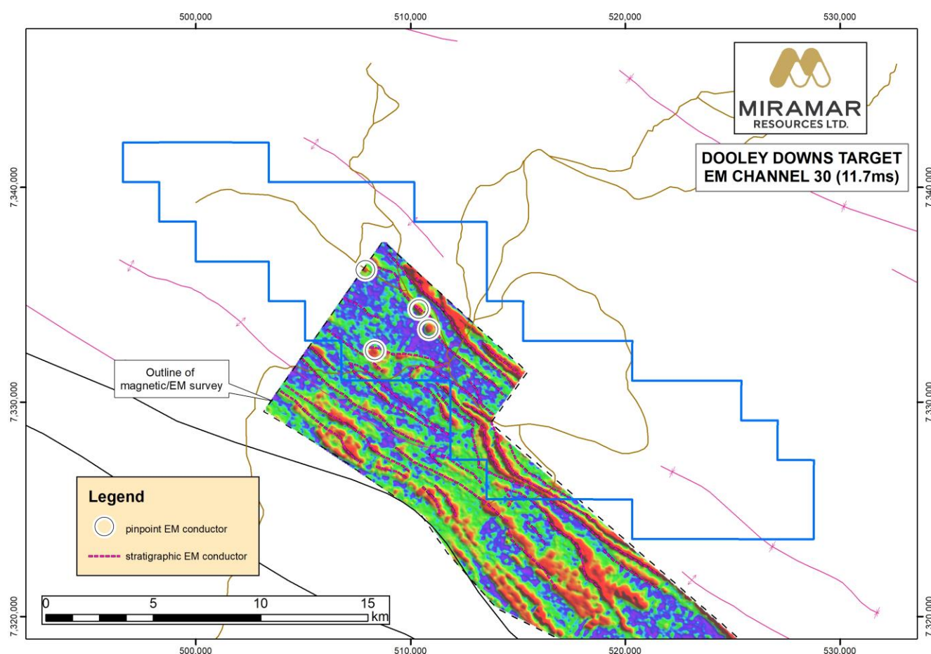
Figure 8. Dooley Downs Target showing location of open file EM/magnetic survey and conductors.
