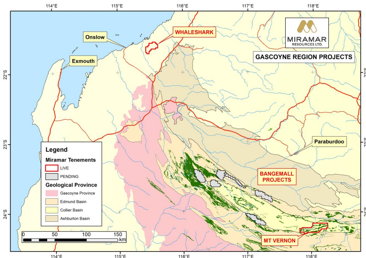
Figure 6. Location map for Miramar's Gascoyne region projects.
