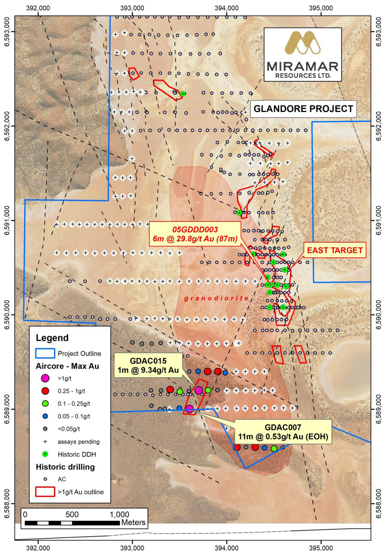
Figure 4. Glandore Project showing recent aircore results and lake drilling.
