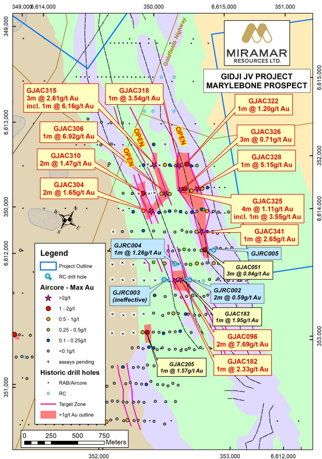
Figure 2. Marylebone Target showing all drilling and significant results to date.
