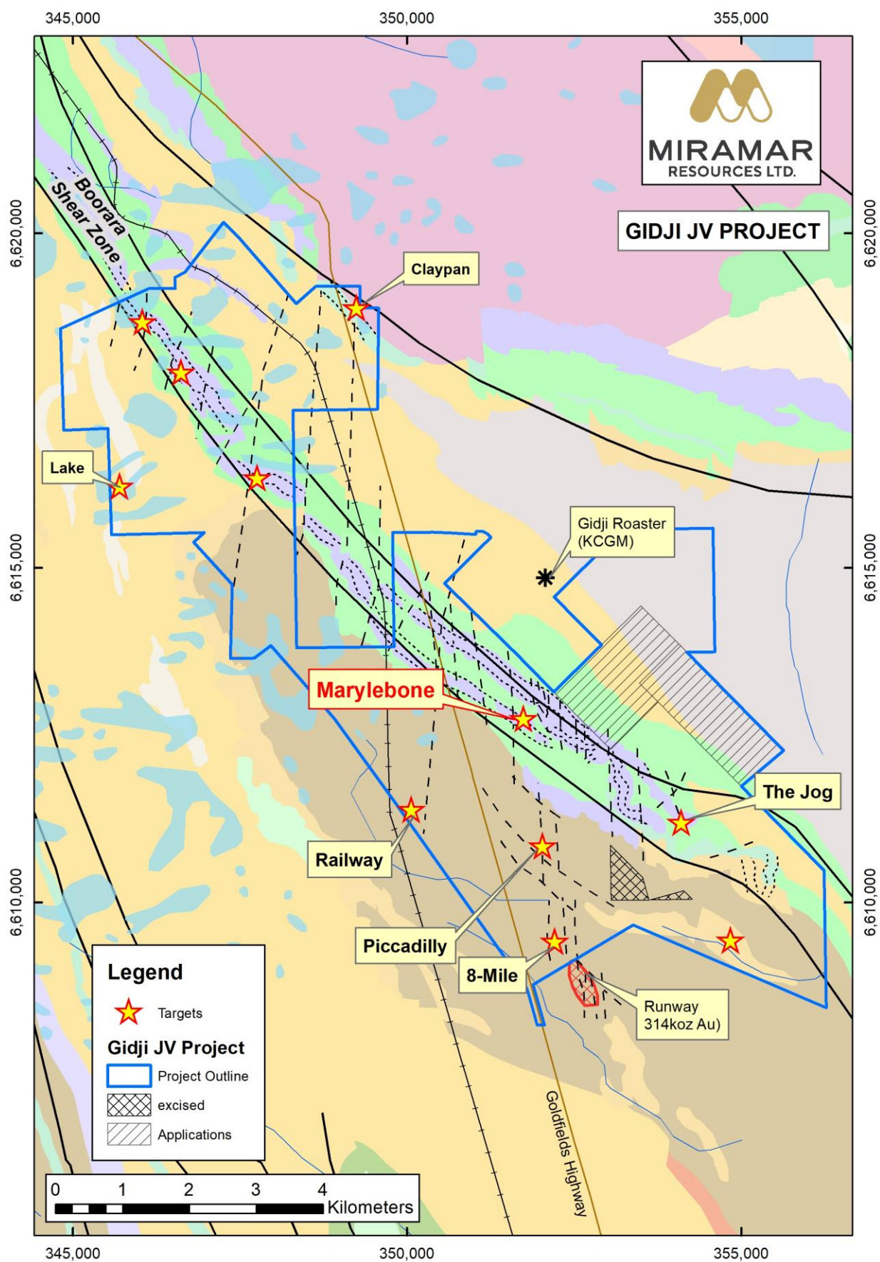
Figure 3. Gidji JV Project showing land position and targets after grant of tenements.
