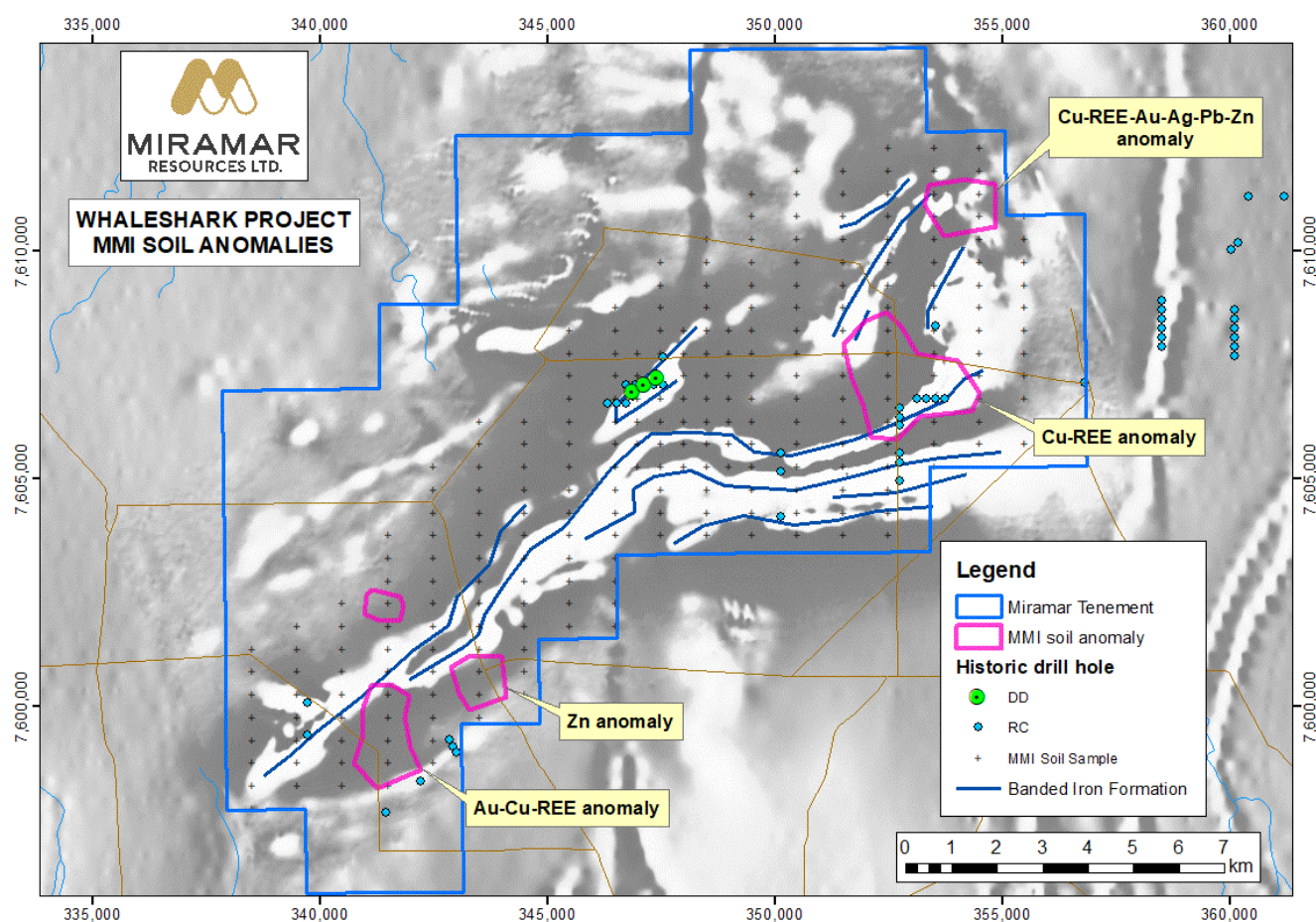
Figure 7. Whaleshark Project showing summary of MMI anomalism over magnetic image.
