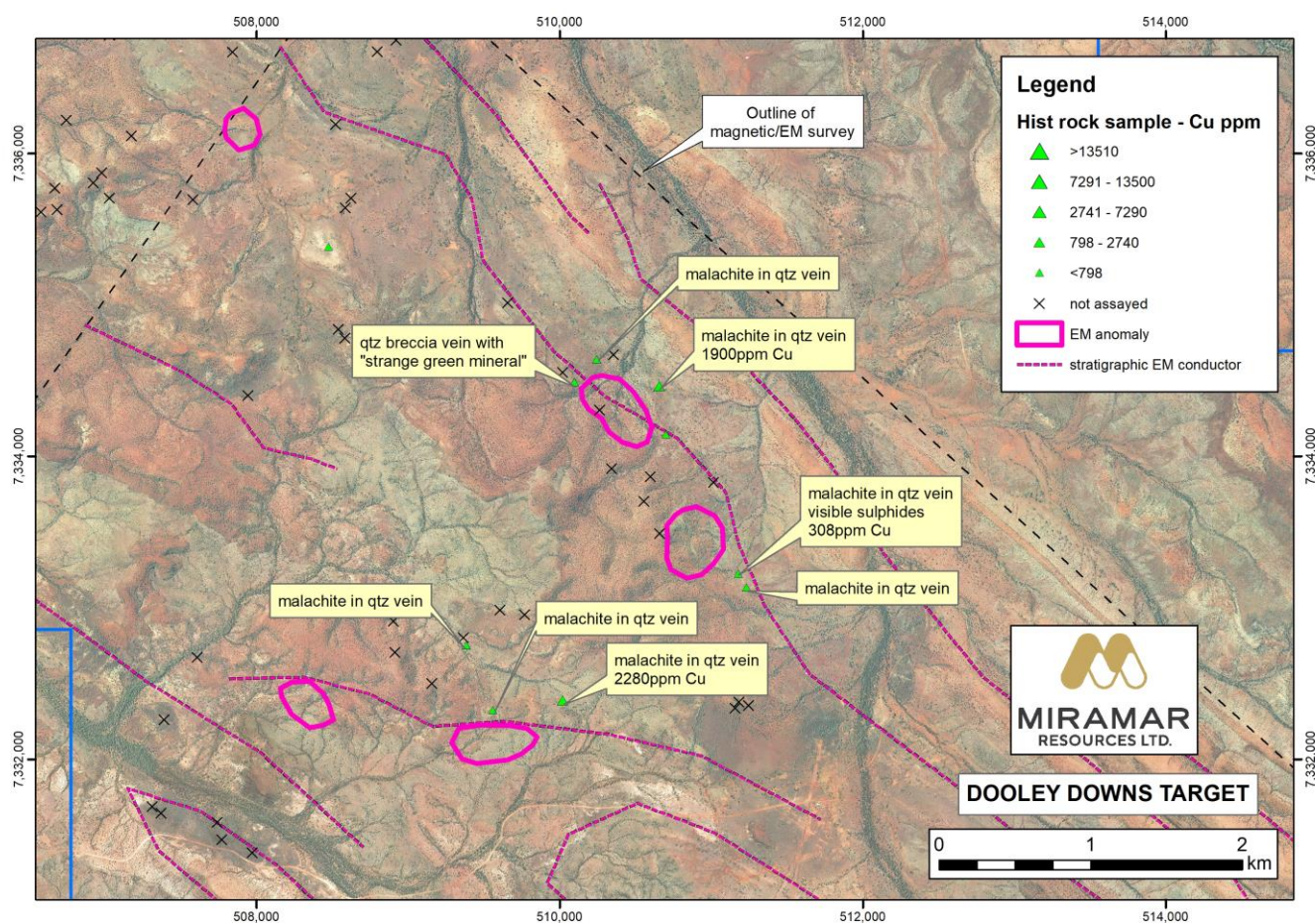
Figure 9. Dooley Downs Target showing location of historic rock samples in relation to EM conductors.
