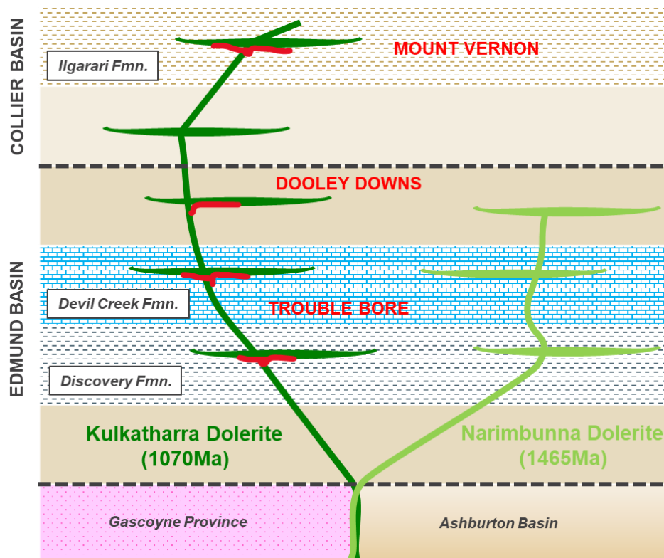
Figure 3. Schematic diagram showing relationship between two families of dolerite sills, sedimentary units of the Edmund and Collier Basins, and the relative position of Miramar's Ni-Cu-Co-PGE targets.
