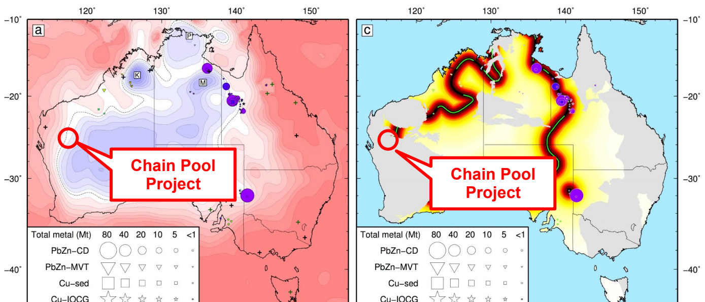
Figure 1. Distribution of sediment-hosted (and IOCG) deposits in relation to lithospheric thickness. (a) Australian Lithosphere/Asthenosphere Boundary (LAB): dashed contour = 170 km LAB depth, (c) Mineral potential heat map based on proximity to the 170 km LAB contour (Czarnota et al, 2020).
