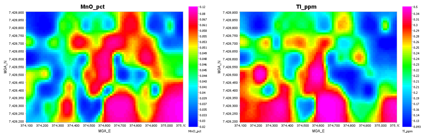
Figure 3. Gridded soil results for MnO and Tl.
