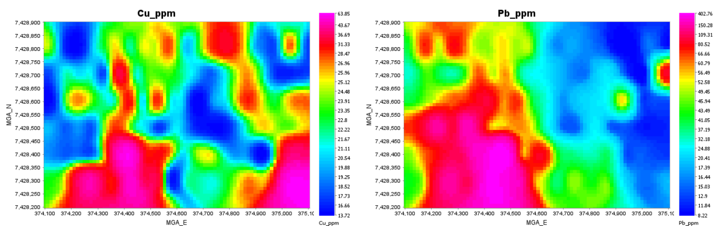
Figure 2. Gridded soil results for Cu and Pb.
