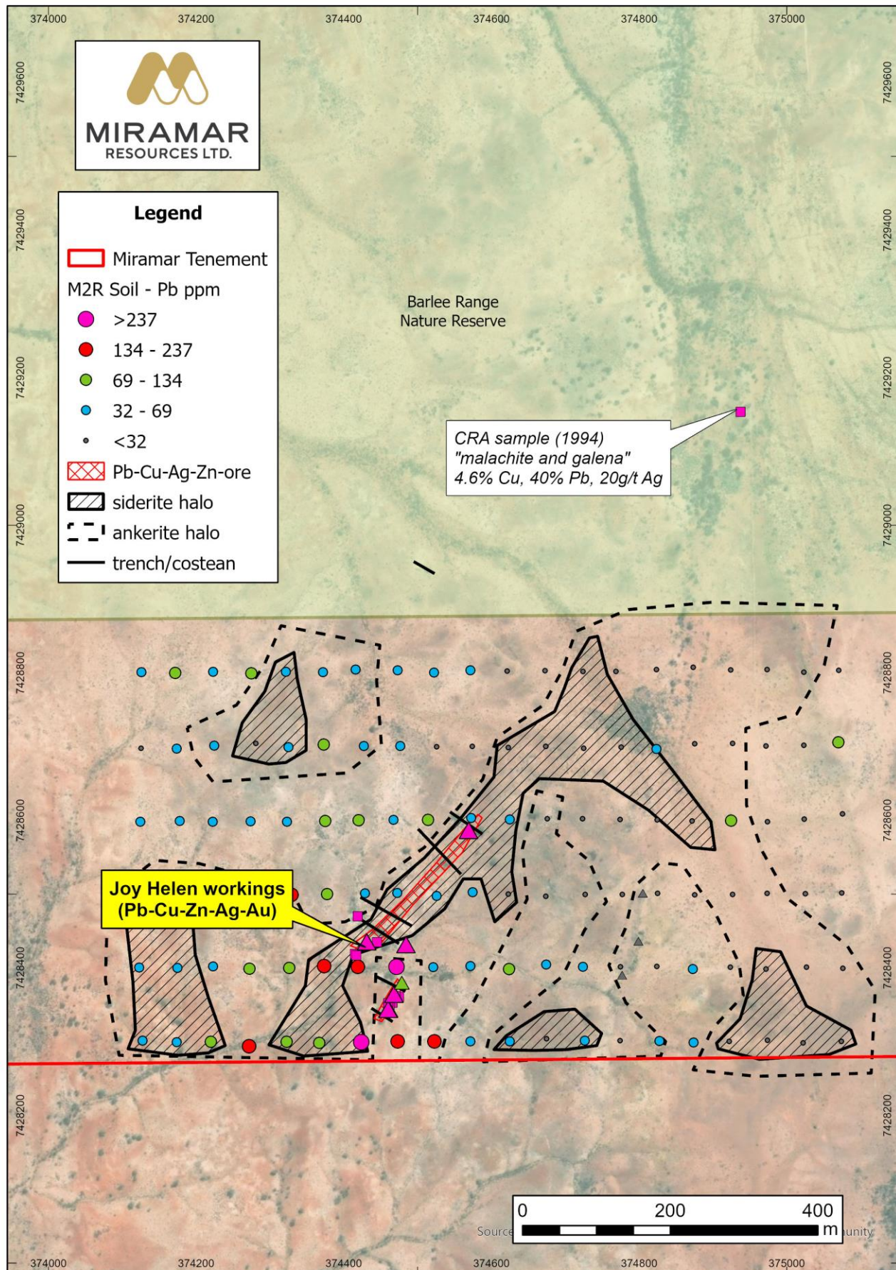
Figure 4. Joy Helen prospect showing carbonate alteration halos and lead (Pb) in soils.
