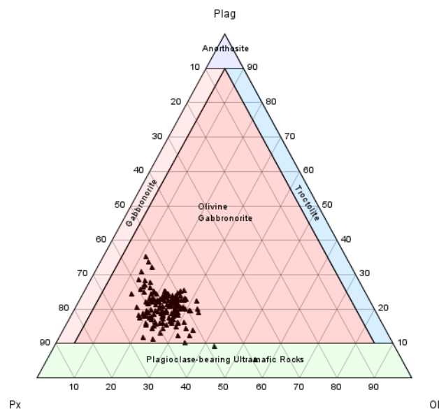
Figure 5. Classification of all 159 samples using olivine(Ol), plagioclase (Plag) and pyroxene (Px), and showing most samples plotting as “olivine gabbro-norite”
