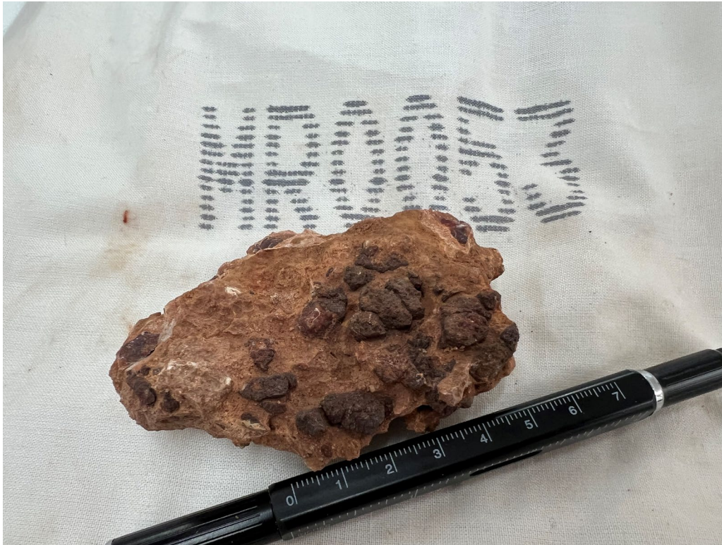
Figure 3. Sample MR0013 (originally MR0053) showing weathered breccia material with dark brown iron-carbonate nodules.
