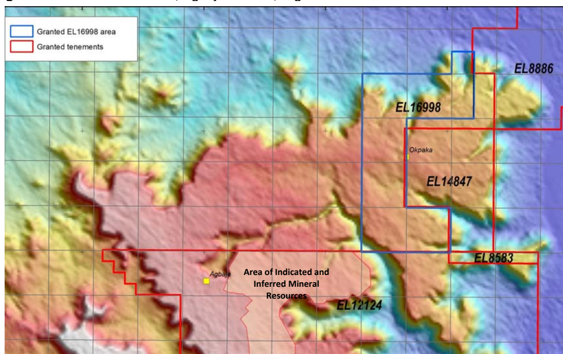
Figure 1: Location of EL16998, Agbaja Plateau, Nigeria
