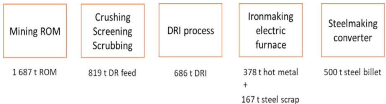
Figure 10 Visualisation of flowsheet
