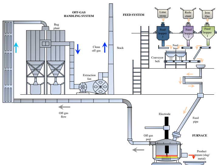
Figure 9 A schematic diagram of the pilot furnace set-up showing the integrated nature of the continuous smelting facility at Mintek (left). The 200 kVA DC arc pilot furnace in operation during the Kogi Iron trial (top right) and metal and slag produced during the trial (bottom right). The crude iron product was used in the oxygen refining development work to demonstrate the successful removal of phosphorus.
