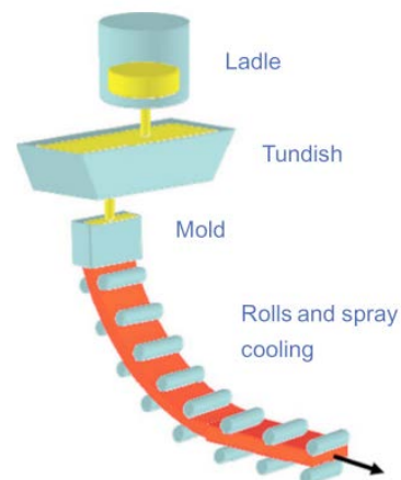
Figure 11 Schematic of a typical continuous casting process (reproduced from Louhenkilpi, 2014)
