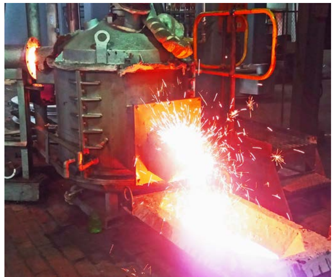
Figure 9 A schematic diagram of the pilot furnace set-up showing the integrated nature of the continuous smelting facility at Mintek (left). The 200 kVA DC arc pilot furnace in operation during the Kogi Iron trial (top right) and metal and slag produced during the trial (bottom right). The crude iron product was used in the oxygen refining development work to demonstrate the successful removal of phosphorus.
