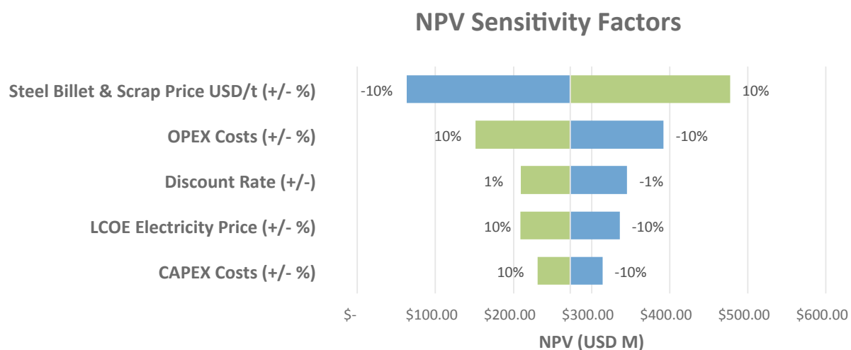
Figure 1: Sensitivity Analysis (after-tax)
