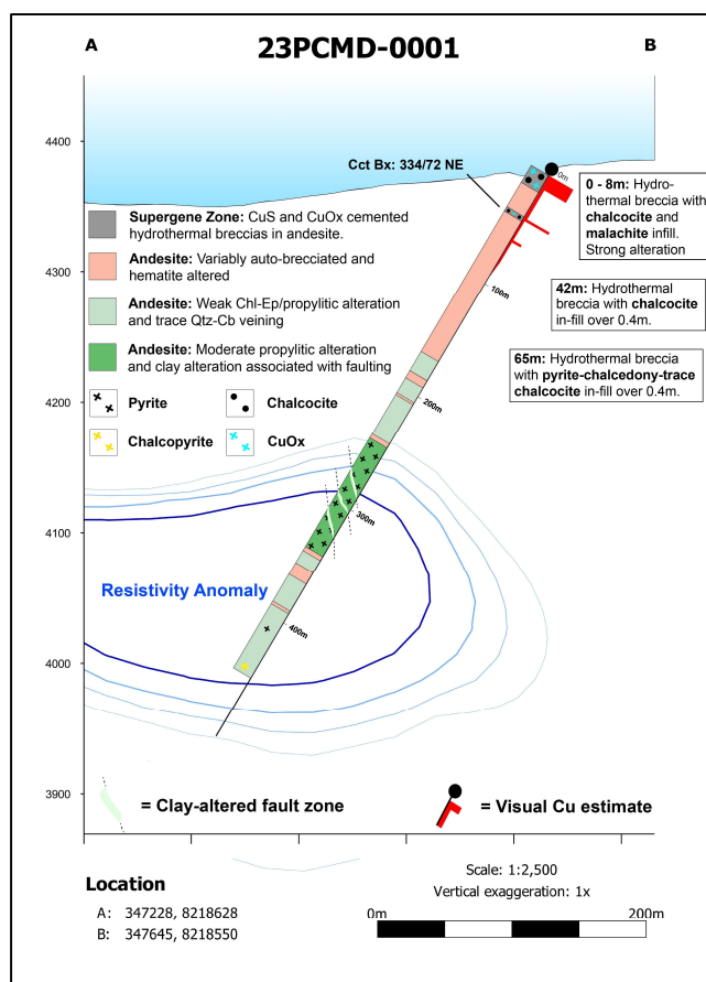
Figure 3: Cross-section of 23PCMD0001, Cobremani Target, with geological interpretation
