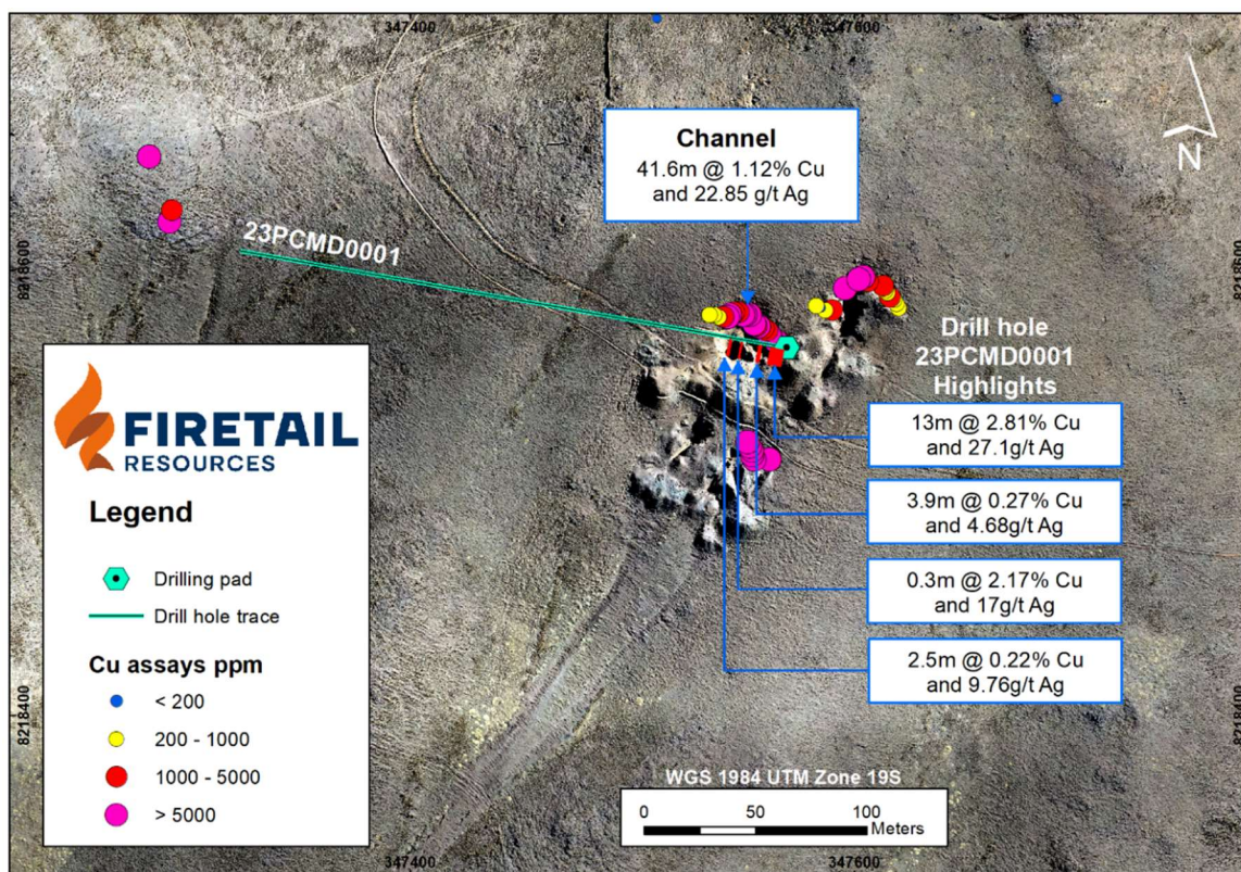
Figure 4: Plan view of 23PCMD0001 at Cobremani target
