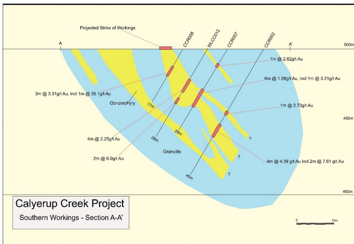
Figure 2 Cross Section through RC drilling at the southern workings
