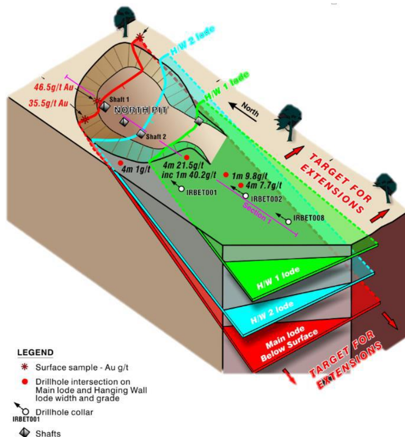
Figure 7 Oblique view of interpreted lodes at Lyndon Bettina
