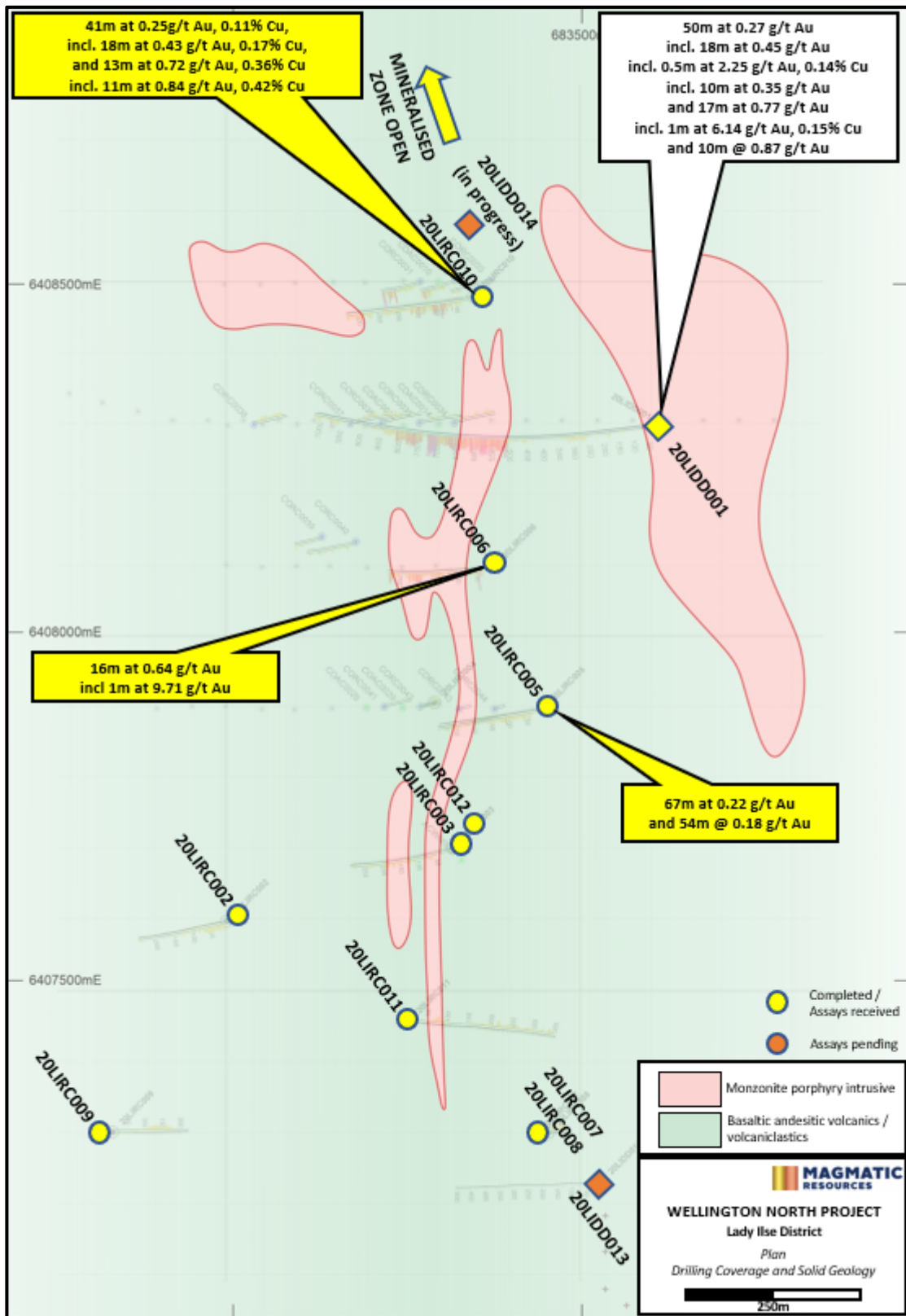
Figure 2: Lady Ilse District, Plan of drilling coverage and solid geology interpretation
