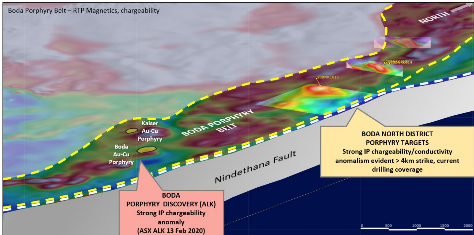
Figure 4: Oblique view of Boda Porphyry Belt, highlighting Boda North targets, characterised by strong chargeability anomalism, showing recent IP survey chargeability depth slice (ASX MAG 1 June 2020) and reprocessed, historical IP chargeability sections
