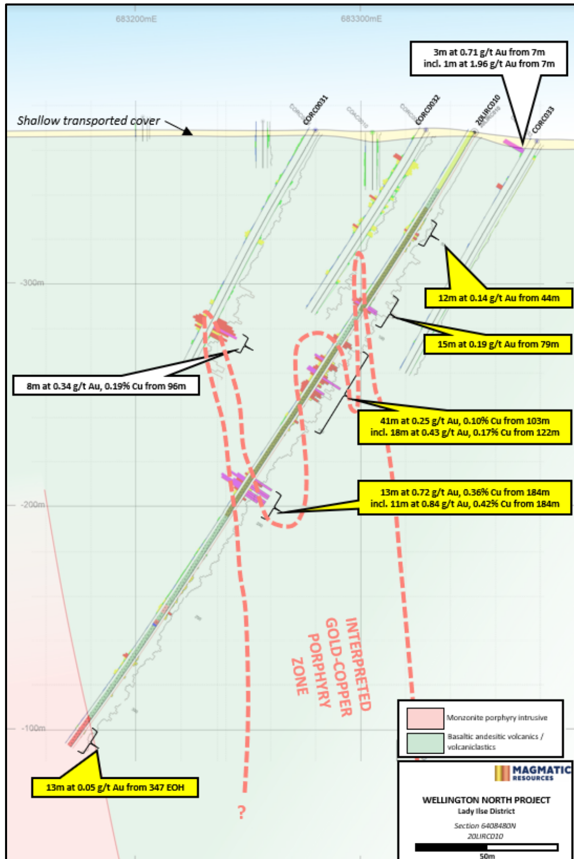
Figure 1: 20LIRC010 Section, looking north
