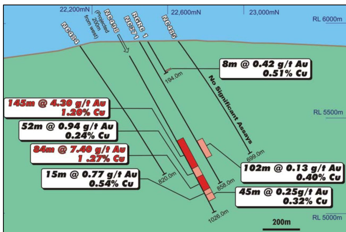
Figure 3: Ridgeway Gold-Copper Porphyry Deposit, discovery drill sequence (Wood 2010)
