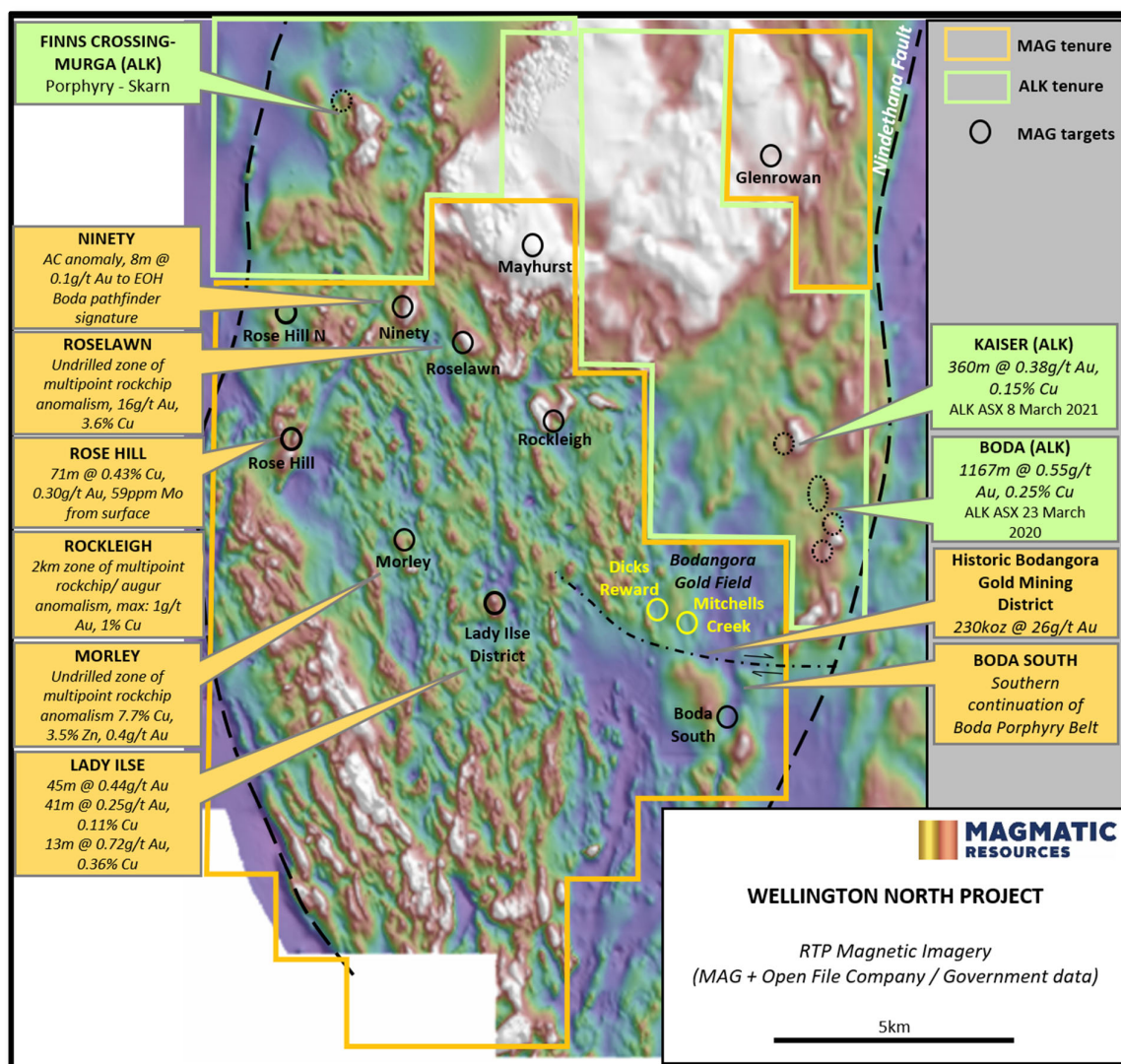
Figure 2: Wellington North Project, Aeromagnetic imagery, RTP (Magmatic and Open File Company/Government) showing northern Molong Belt summary target portfolio, highlighting Boda Au-Cu Discovery (ASX:ALK)
