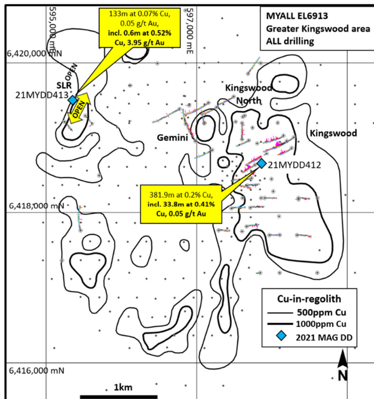
Figure 3: Myall Project, Kingswood District, showing drilling coverage and regolith Cu anomalism
