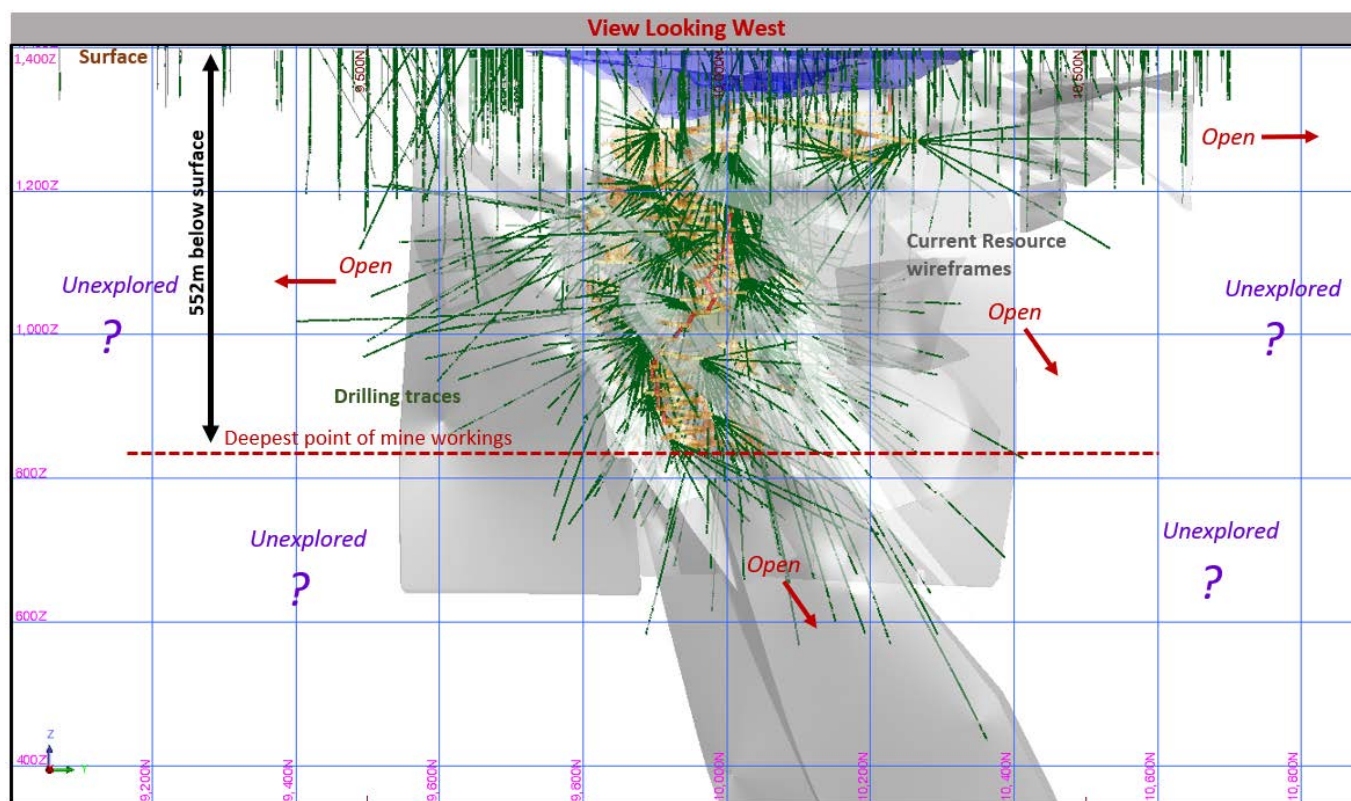
FIGURE 4: Red October, Longitudinal Section showing existing resource wireframes, drilling and mine workings (RO mine grid co-ordinates)
