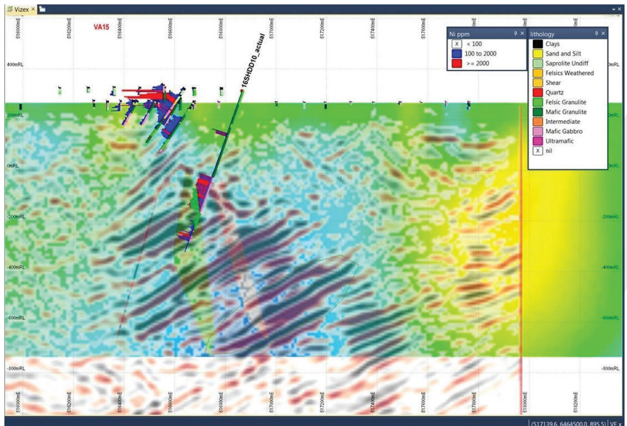
FIGURE 22: Symons Hill Project Seismic Section SLO1 showing trace of diamond drill hole SHDD10 and distinctive seismic survey results. (Drill hole projected approximately 200 metres onto cross section)
