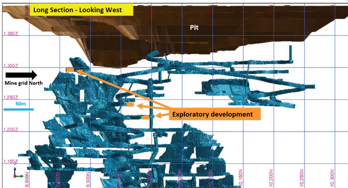
FIGURE 8: Exploratory development during FY2019
