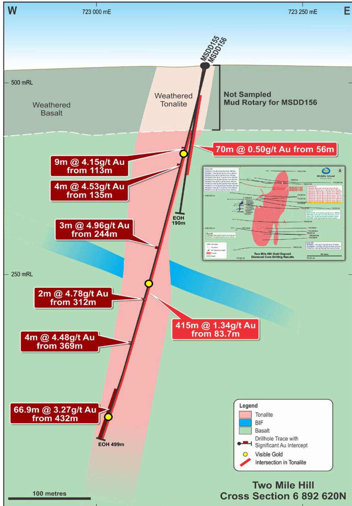
Figure 7. Two Mile Hill diamond drill section 6,892,620N.
