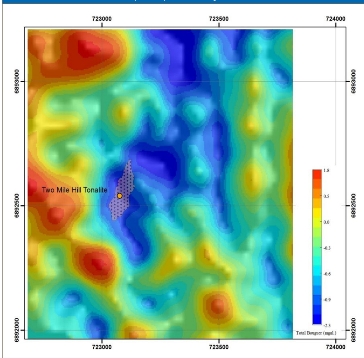
Figure 9. Ground gravity image showing the Two Mile Hill tonalite and several possible proximal analogues (darker blue).
