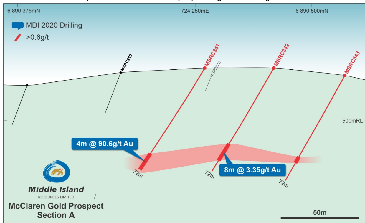
Figure 4 Oblique-Section A - McClaren Prospect, showing new RC drilling results
