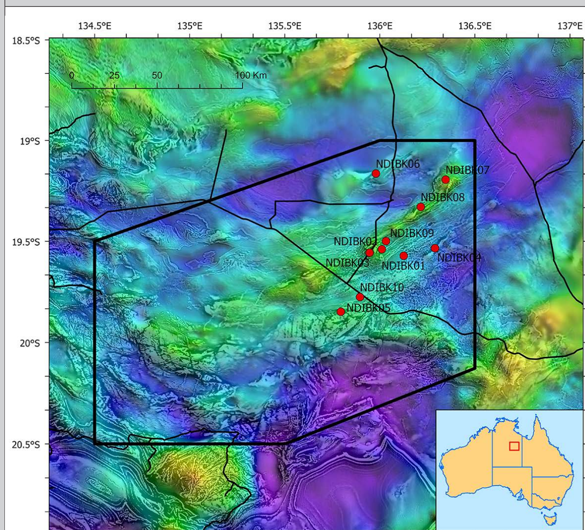
Figure 5. East Tennant borehole locations completed by Minex CRC - base layer is gravity coverage, draped over the first vertical derivative magnetic coverage.
