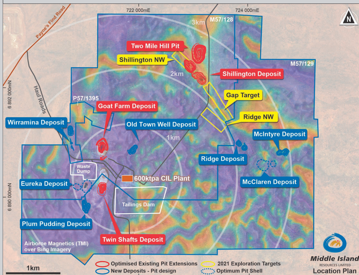
Figure 7. Sandstone Gold Project - Open pit gold deposits and targets assessed in 2020/21.
