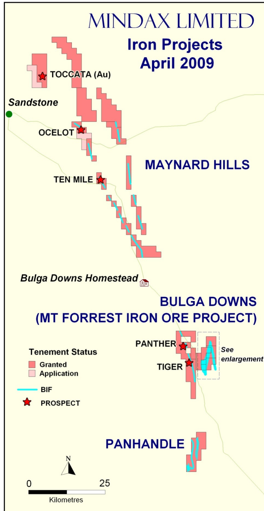
Figure 5: Iron Prospects Sandstone to Mt Forrest
