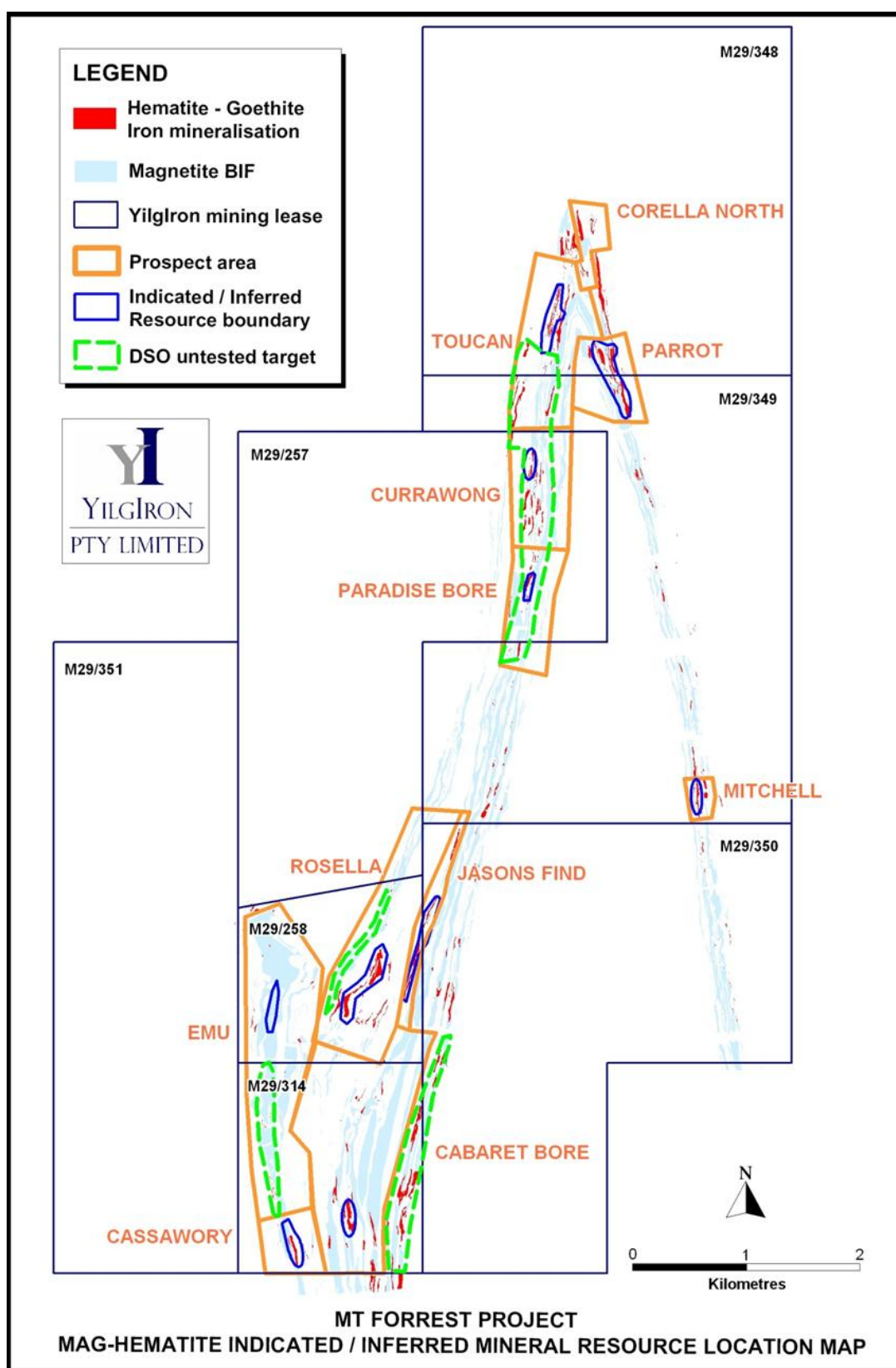
Figure 1 Mt Forrest Oxidised Iron mineralisation location map
