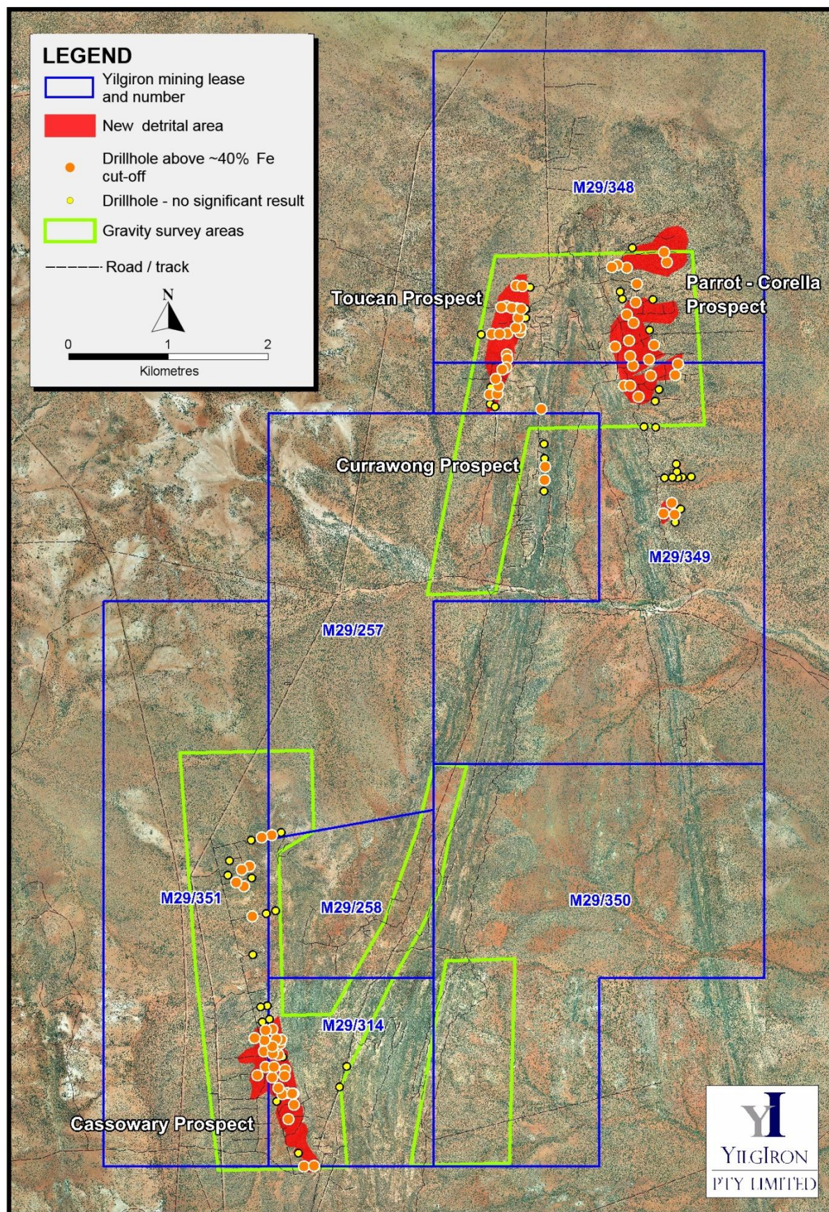
Figure 4: Drilled detrital iron occurrences at Mt Forrest
