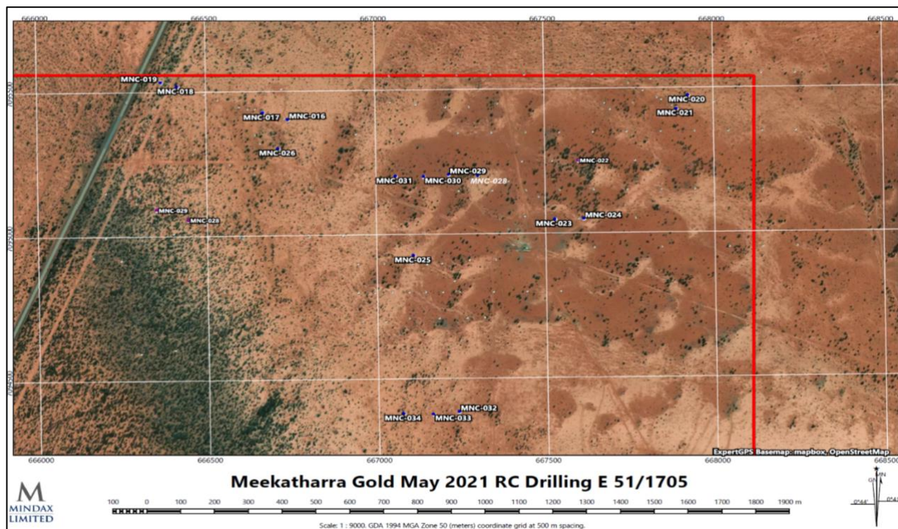
Figure 2: Collar Location Plan with Northern Tenement boundary.
