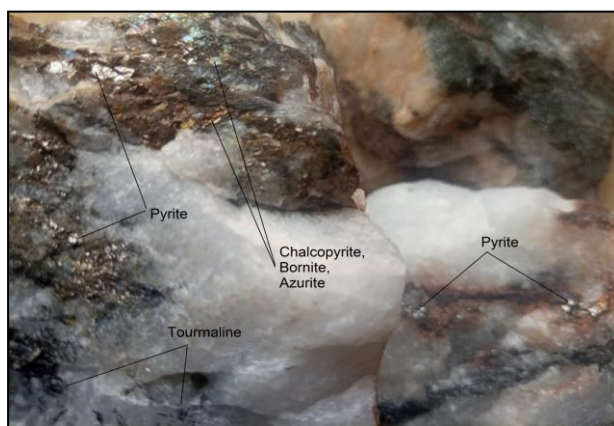
Figure 8 – Close-up of vein from CKTR003 – tourmaline and chalcopyrite, bornite, azurite bearing quartz vein with relicts of host rock
