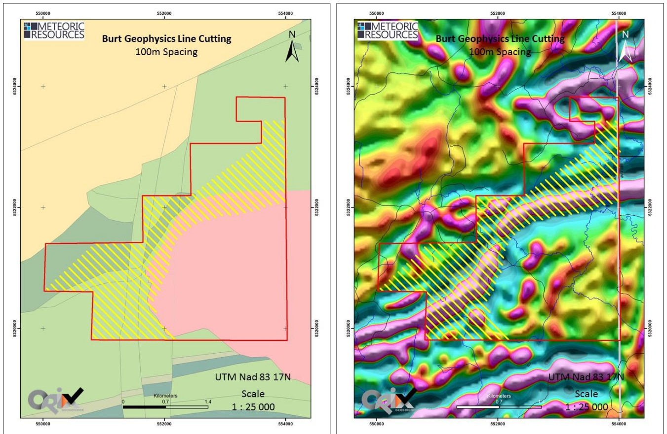
Figure 5: Finalised 100m spaced IP/Magnetics/Resistivity ground-based geophysics program for Burt Cobalt Project
