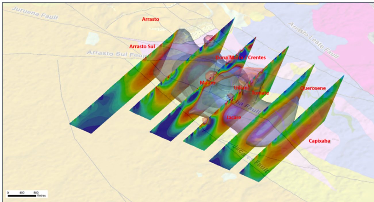
Figure 5: 2D sections showing chargeability (inversions) with 3D Voxel model overlaid. The 3D Voxel model in the diagram represents bodies with values >10mv/v and >15mv/v and signifies a major chargeability anomaly situated close to the Gleba Fault between the Juruena Fault to the North and the Jacares Fault to the south. The anomaly strengthens again and remains open to the north-west beneath the Arrasto Hills Volcanics.
