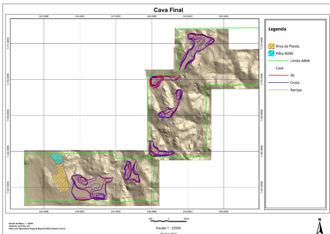
Figure 6: Pit Designs Capão do Mel and Soberbo with plant site in yellow
