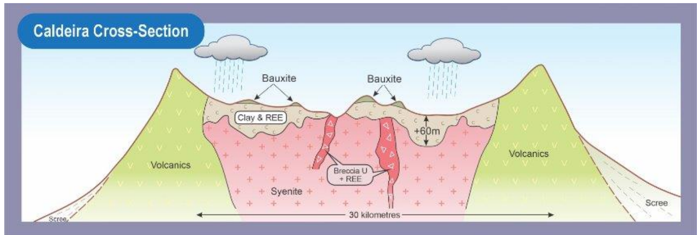
Figure 3: Illustration of the weathering formation of the Caldeira ionic clay deposit
