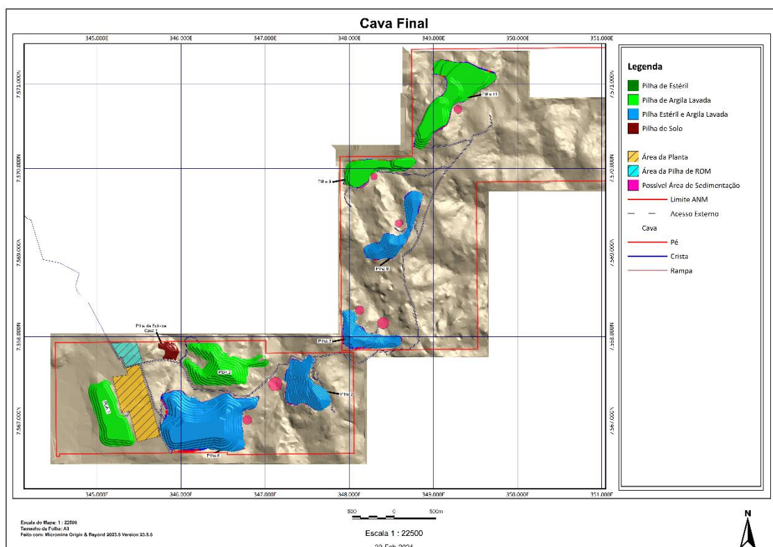
Figure 7: Final Pits showing dry stacked and backfilled pit areas in Blue and Green. Plant site area in yellow.
