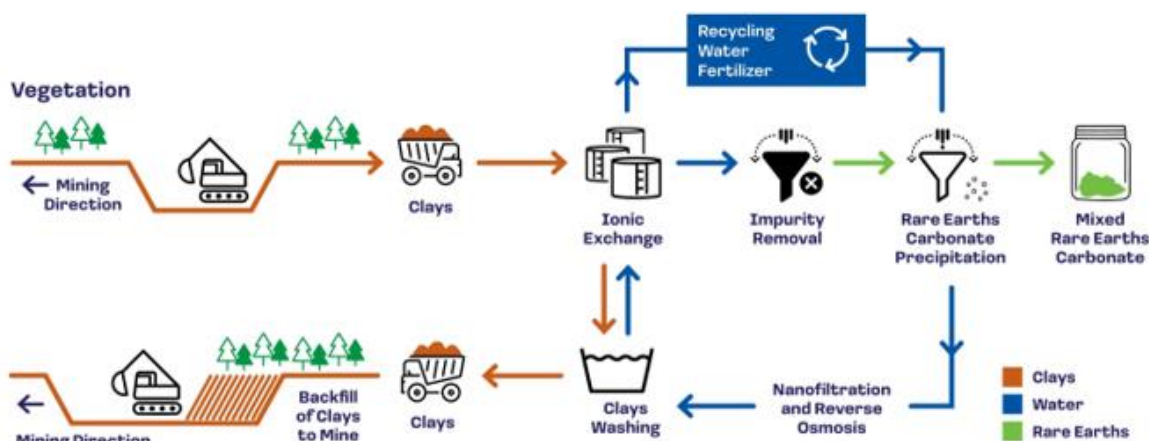
Figure 9: Simple process flowsheet
