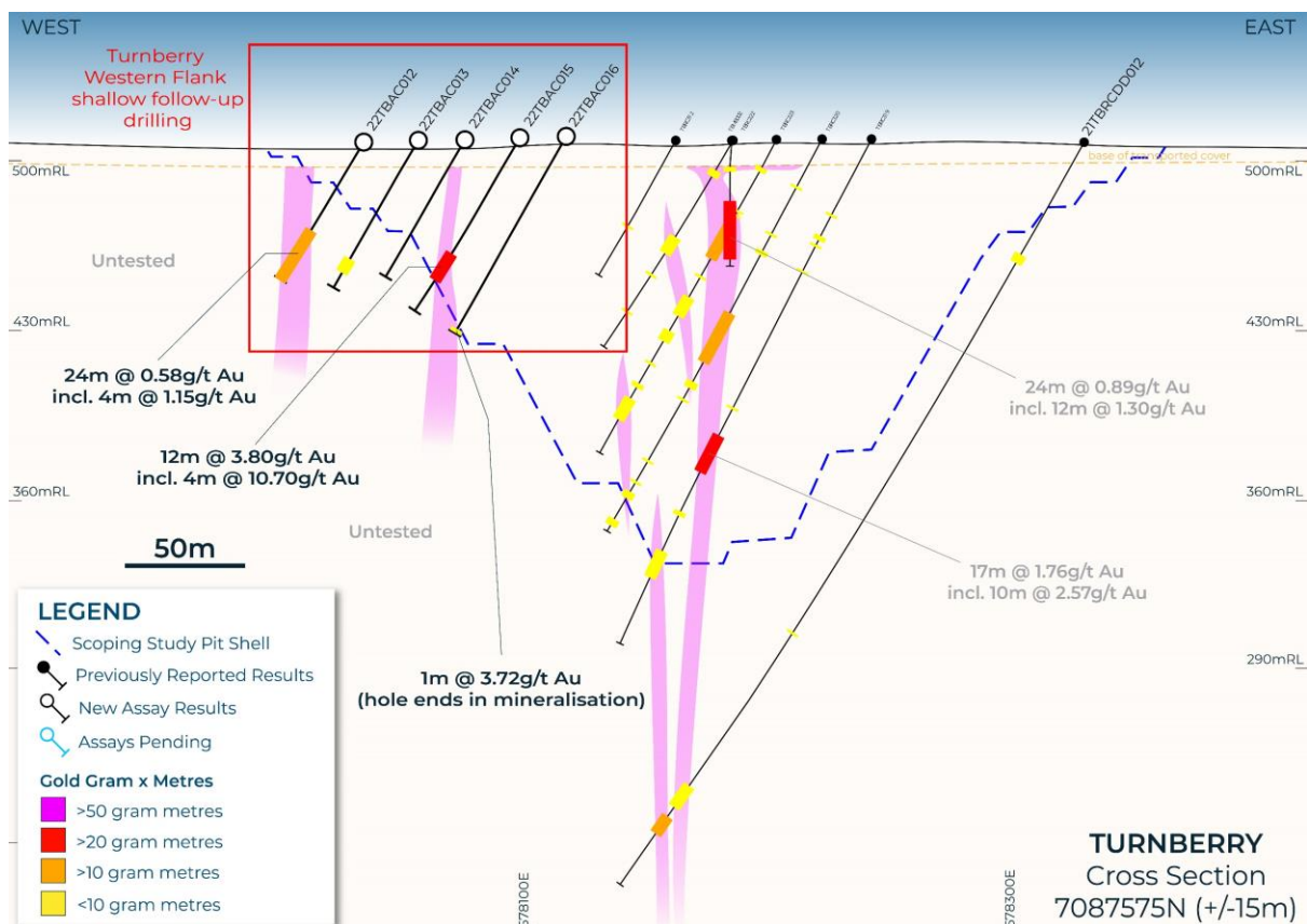
Figure 4: Cross section 7087575N showing hole locations and results, and simplified Scoping Study pit shell. Note the Western Flank mineralisation is yet to be included in the current Mineral Resource.
