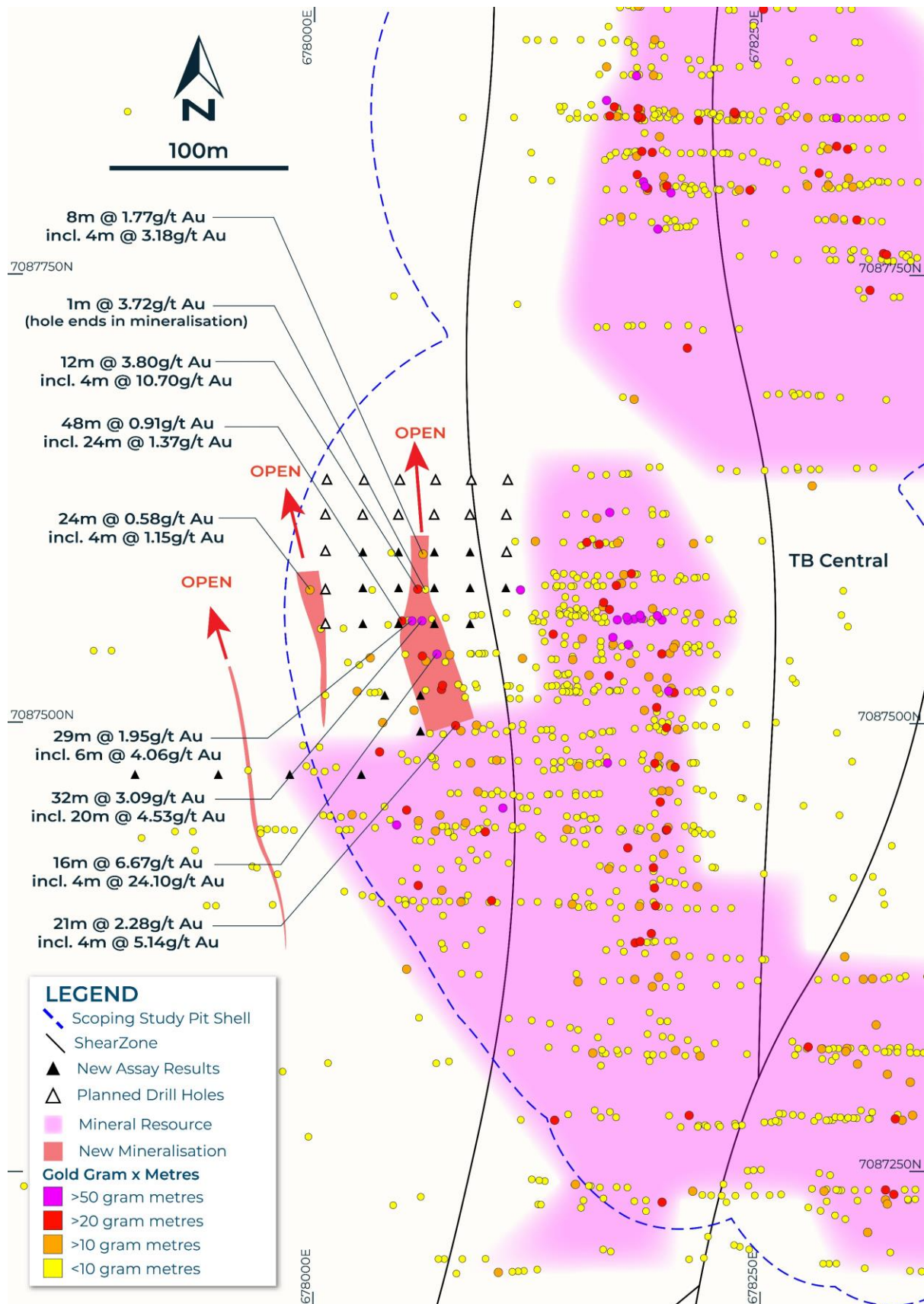
Figure 2: Plan showing interpreted shallow high-grade gold mineralisation intersected on the Western Flank.
