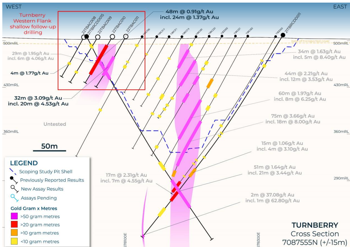
Figure 3: Cross section 7087555N showing hole locations and results, and simplified Scoping Study pit shell. Note the Western Flank mineralisation is yet to be included in the current Mineral Resource.
