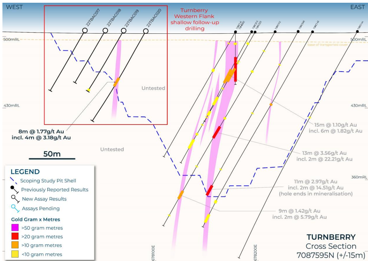
Figure 5: Cross section 7087595N showing hole locations and results, and simplified Scoping Study pit shell. Note the Western Flank mineralisation is yet to be included in the current Mineral Resource.
