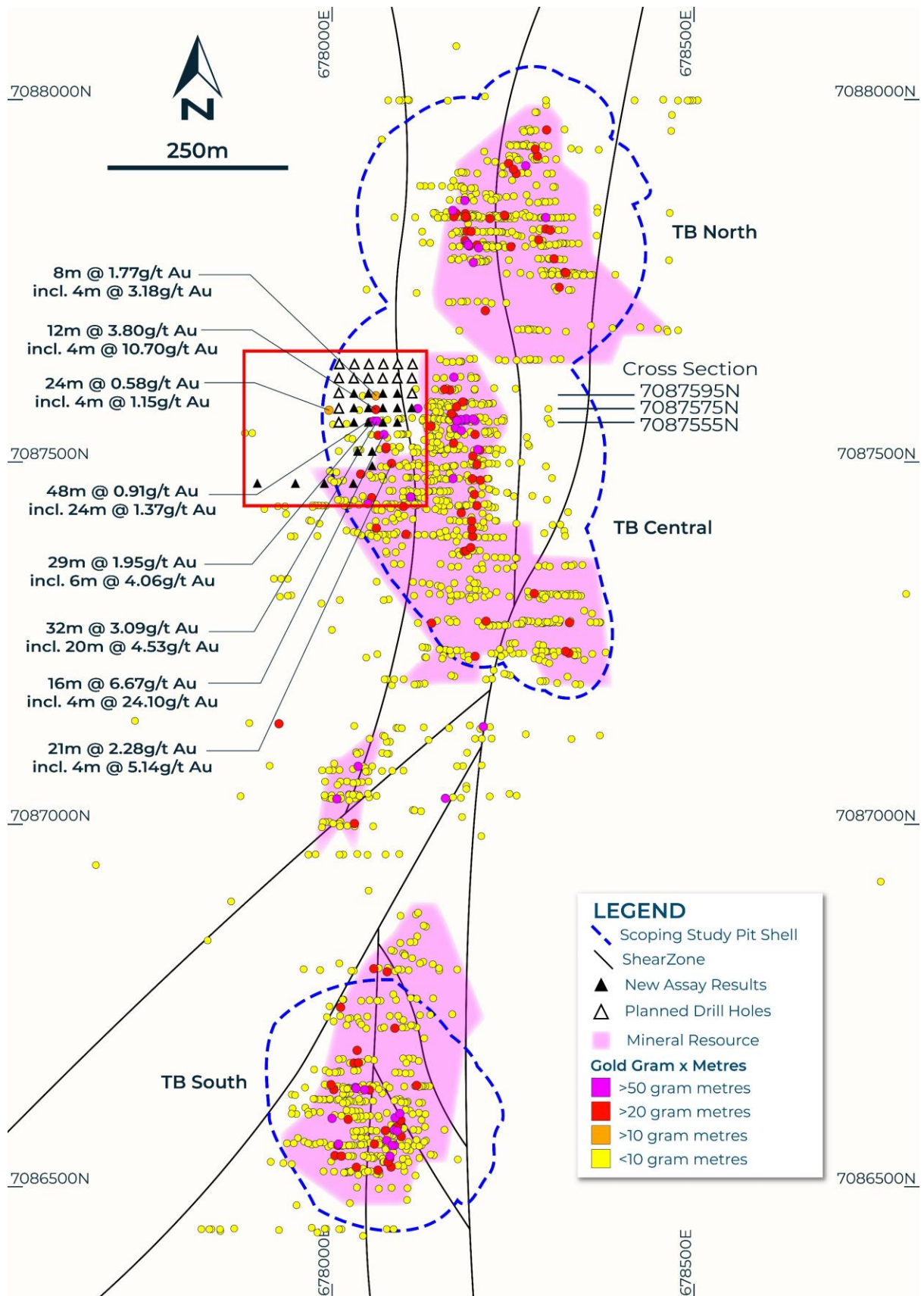
Figure 1: Plan showing Western Flank hole locations and results, current Mineral Resource and Scoping Study pit shell. Position of cross sections (Figure 3, 4 & 5) is shown on right hand side of Turnberry Central.
