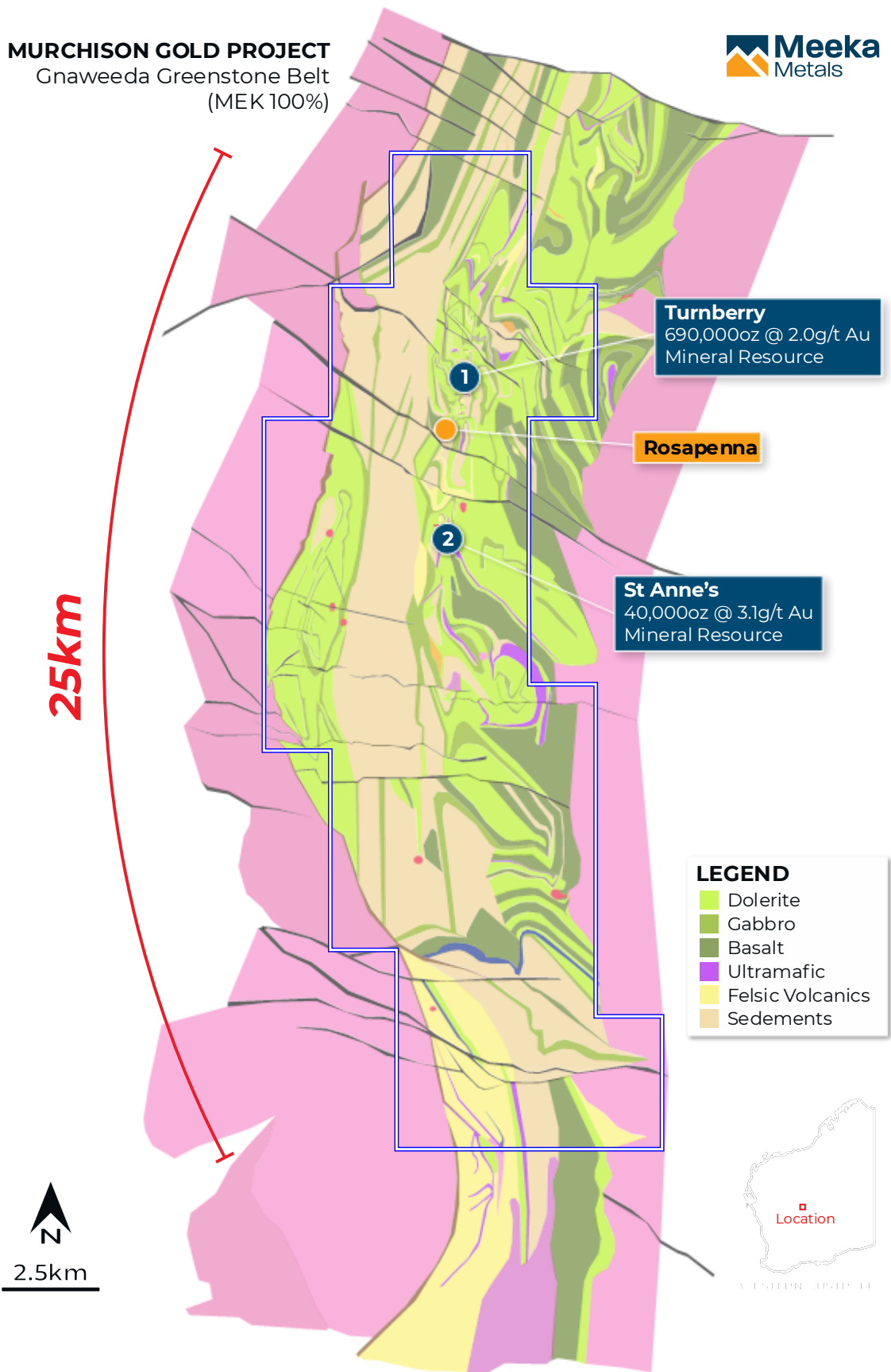
Figure 3: Plan showing ~25km belt of highly prospective Archean greenstones that forms part of Meeka's Murchison Gold Project and is currently being systematically drill tested.
