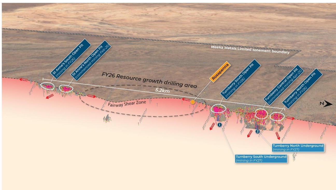
Figure 4: Long section showing the prospective Fairway shear zone between Turnberry and St Anne's where first pass drilling has commenced and gold has been intersected at Rosepenna.
