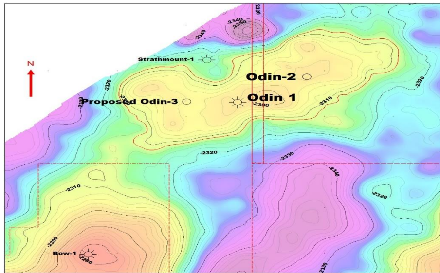
Toolachee formation depth map Odin gas field
