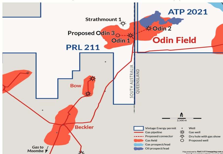
Odin field location map with connection to Vali-Beckler pipeline
