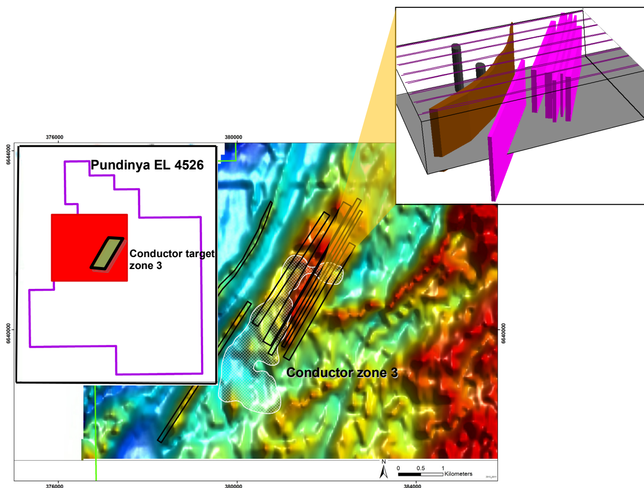
Figure 2: Durkin – conductor 3 target zone area magnetic anomaly image with outline of AEM anomaly overlain (white stipple). Modeled bodies for drill testing associated with anomalous conductive and gravity results inset (pink shapes).
