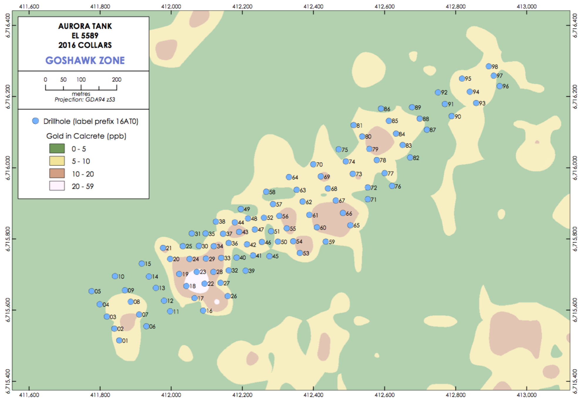
Figure 3: 2016 Drilling Goshawk Gold Prospect – Location of drillhole collars
