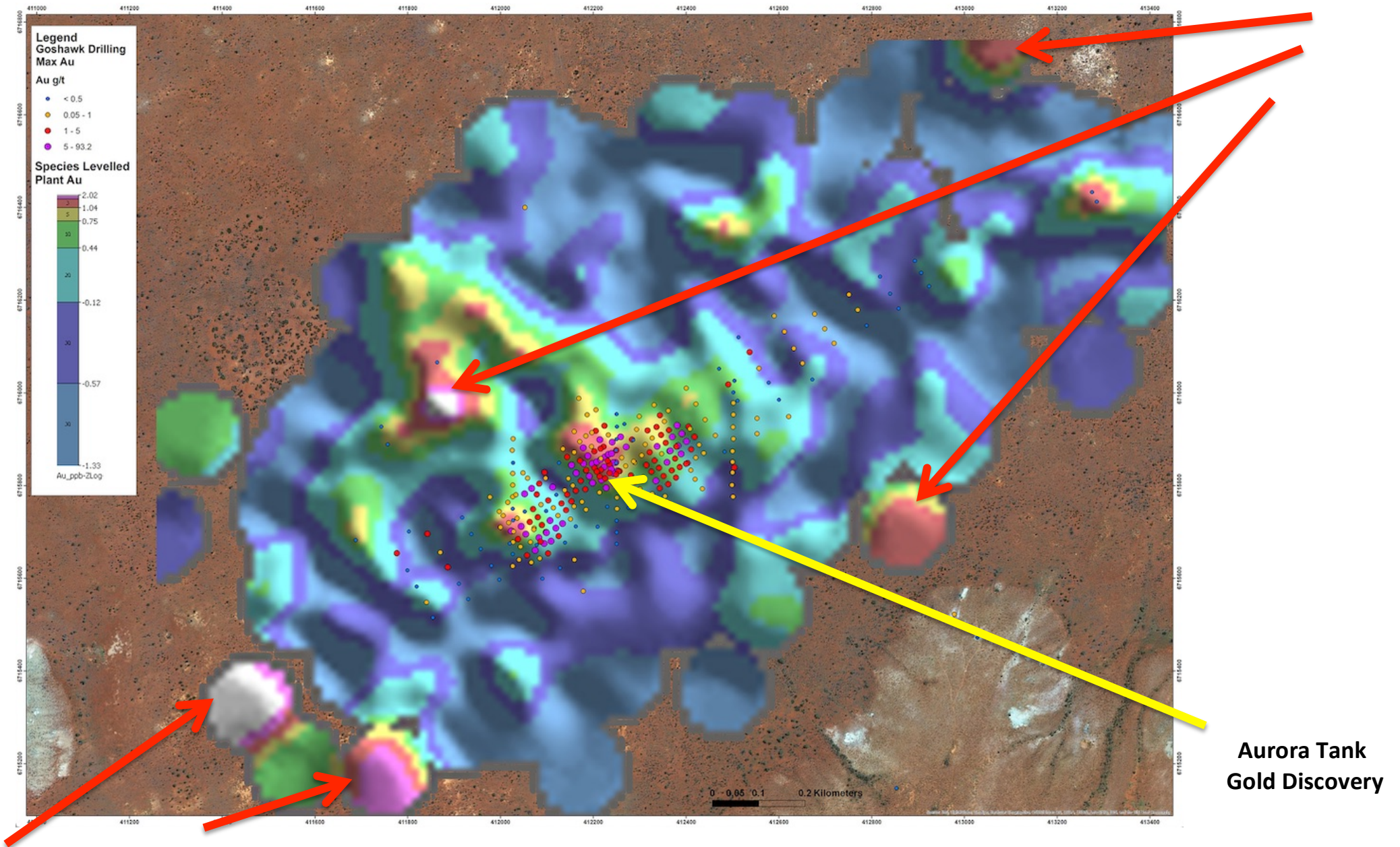
Figure 3: Aurora Tank – Gold biogeochem contours + drillhole gold assays g/t ••
