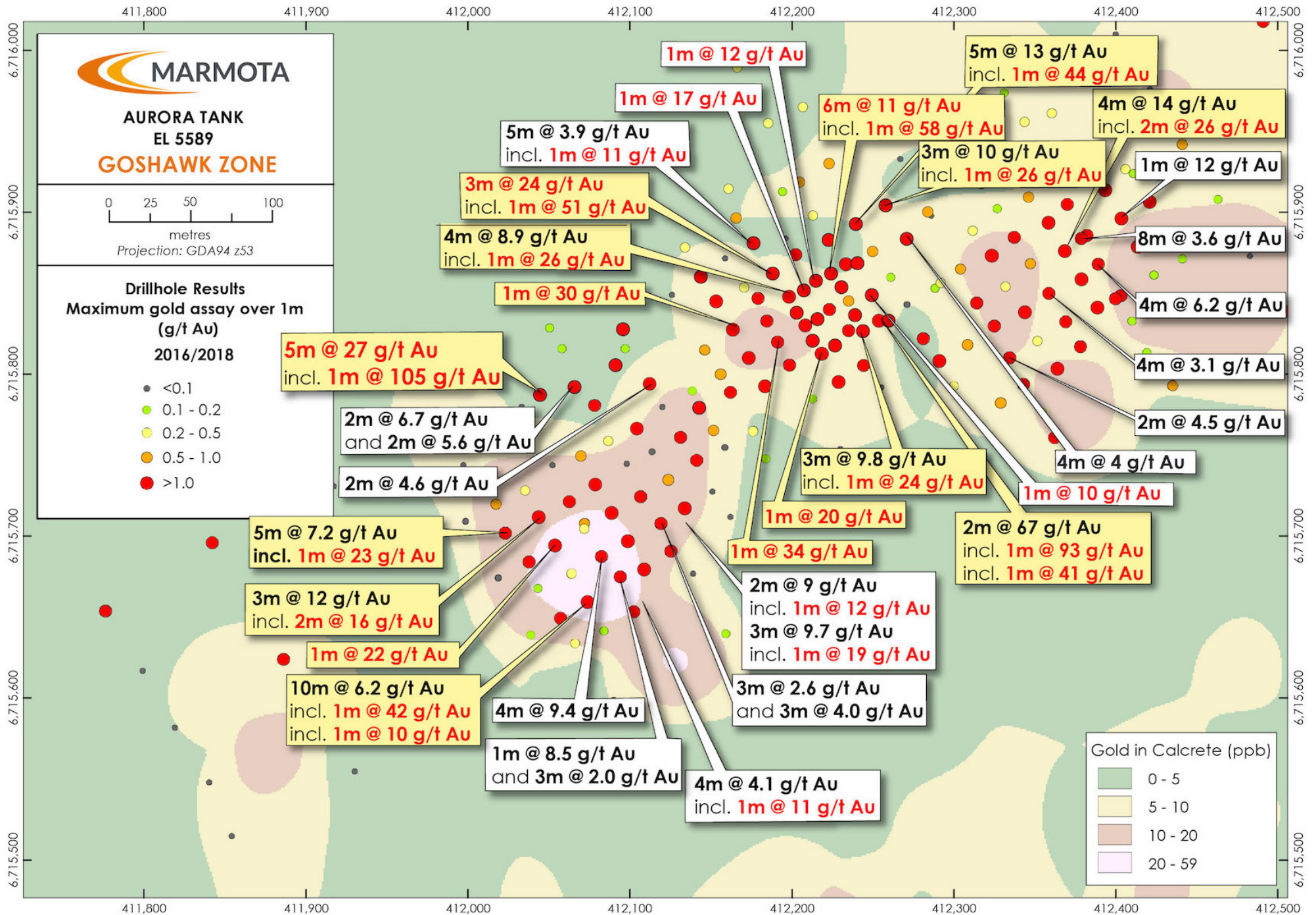
Figure 4: Aurora Tank – Best downhole gold results
