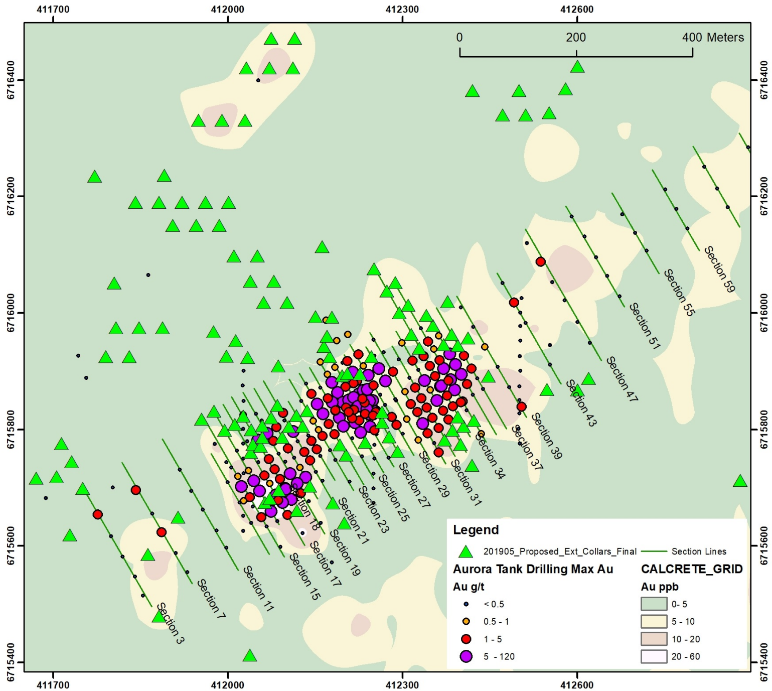
Figure 2: Aurora Tank Phase 1 planned June 2019 AC holes ▲
