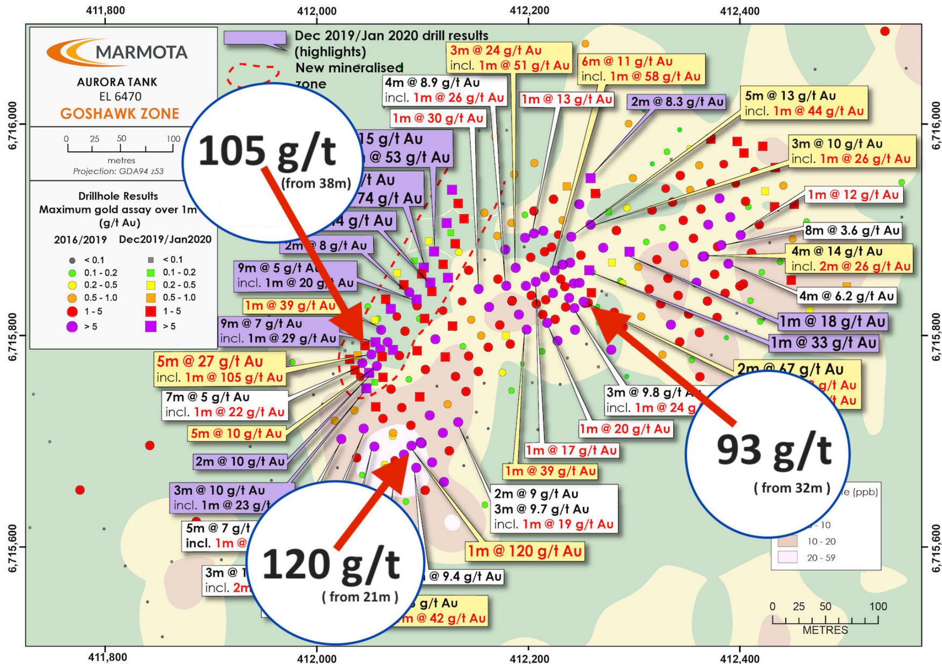
Figure 1: Aurora Tank Gold discovery – Best downhole gold results
