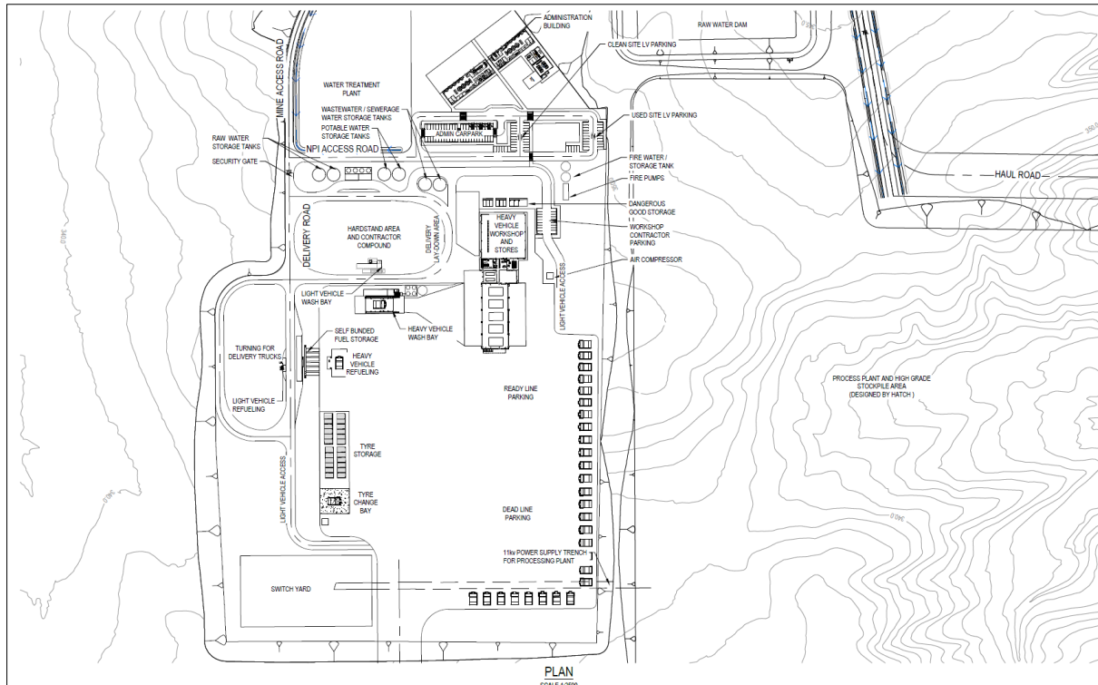
Figure 2. Non-Process Infrastructure - Workshops, administration and hardstand - general arrangements
