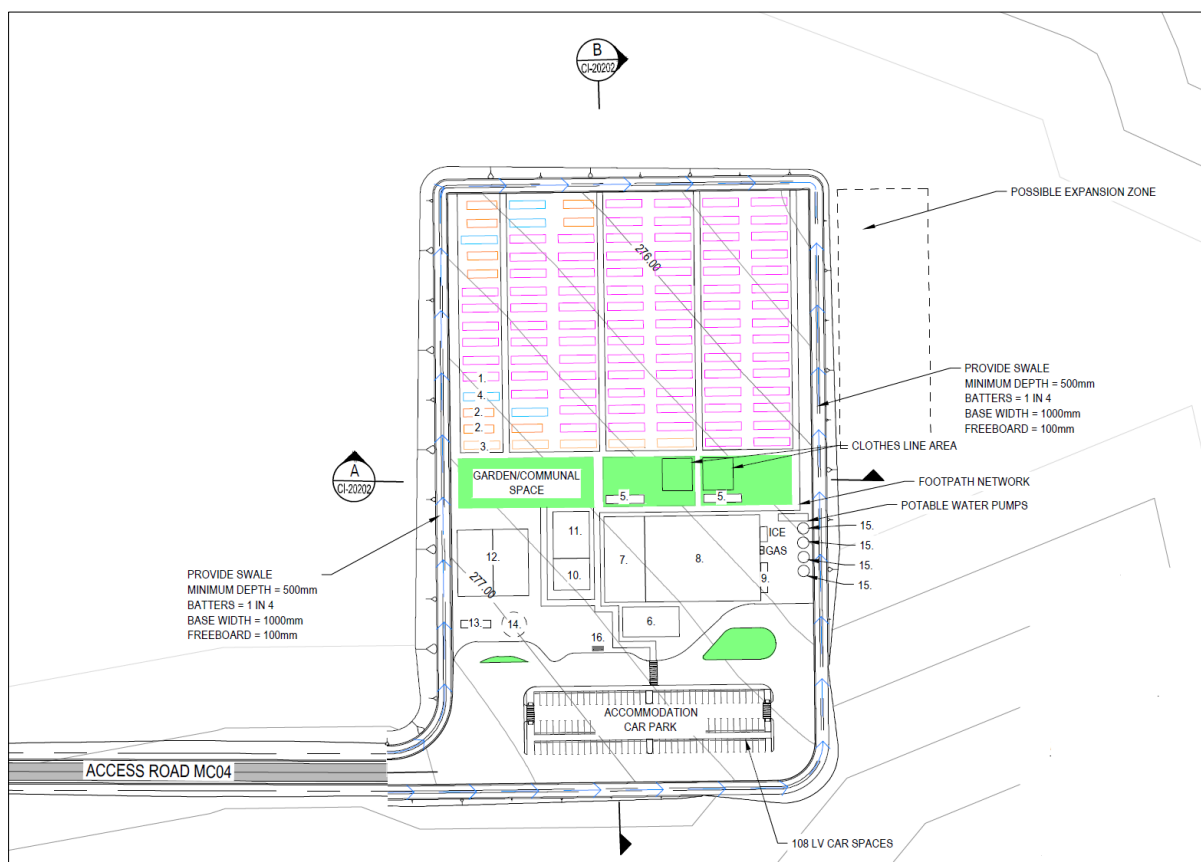
Figure 3. Accommodation/Site Camp layout for expanded Project scale configuration.
