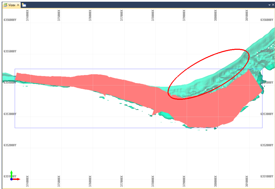
Figure 9. Plan View Razorback resource block modelling (pink) over 0.1 SI unit cutoff geophysical model (green). Unaccounted mineralisation (red ellipse)
