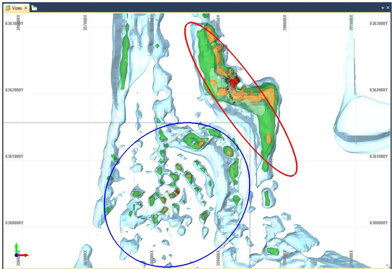
Figure 1: Magnetic modelling showing Manunda Creek (red) and Manunda Hill (blue). 3D shells: 0.1 SI unit cutoff – Blue; 0.25 SI unit cutoff – Green; 0.4 SI unit cutoff– Orange; 0.6 SI unit cutoff – Red
